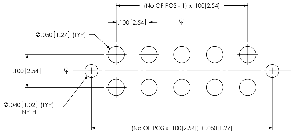
LAYOUT FOR PGP-105-01-X-D-AD SHOWN ALL DIMENSIONS ARE SYMMETRIC ABOUT THE CENTERLINE.
