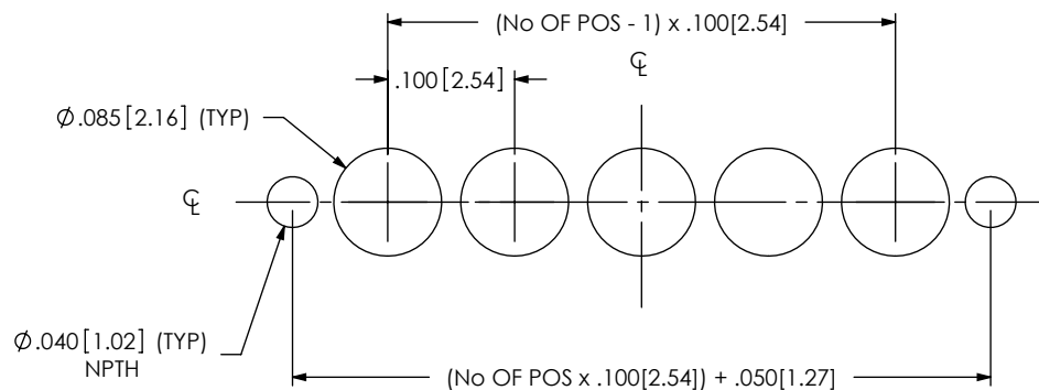
LAYOUT FOR PGP-105-01-X-S-AD SHOWN ALL DIMENSIONS ARE SYMMETRIC ABOUT THE CENTERLINE.
