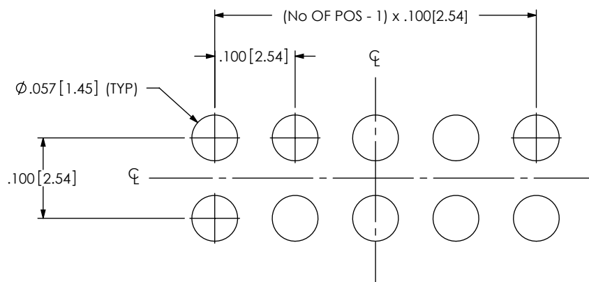
LAYOUT FOR PGP-105-01-X-D-AD SHOWN ALL DIMENSIONS ARE SYMMETRIC ABOUT THE CENTERLINE.
