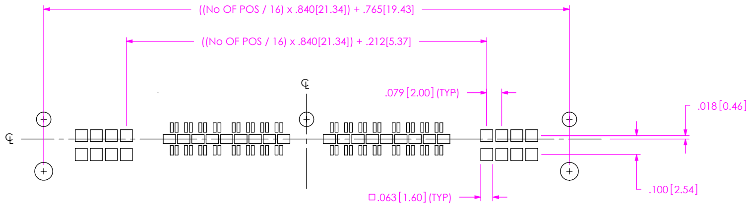
FIG 6 (QFS-032-01-XX-D-DP-RA-PC8 SHOWN) (DIFFERENT AS SHOWN, OTHERWISE SAME AS FIG 2)
