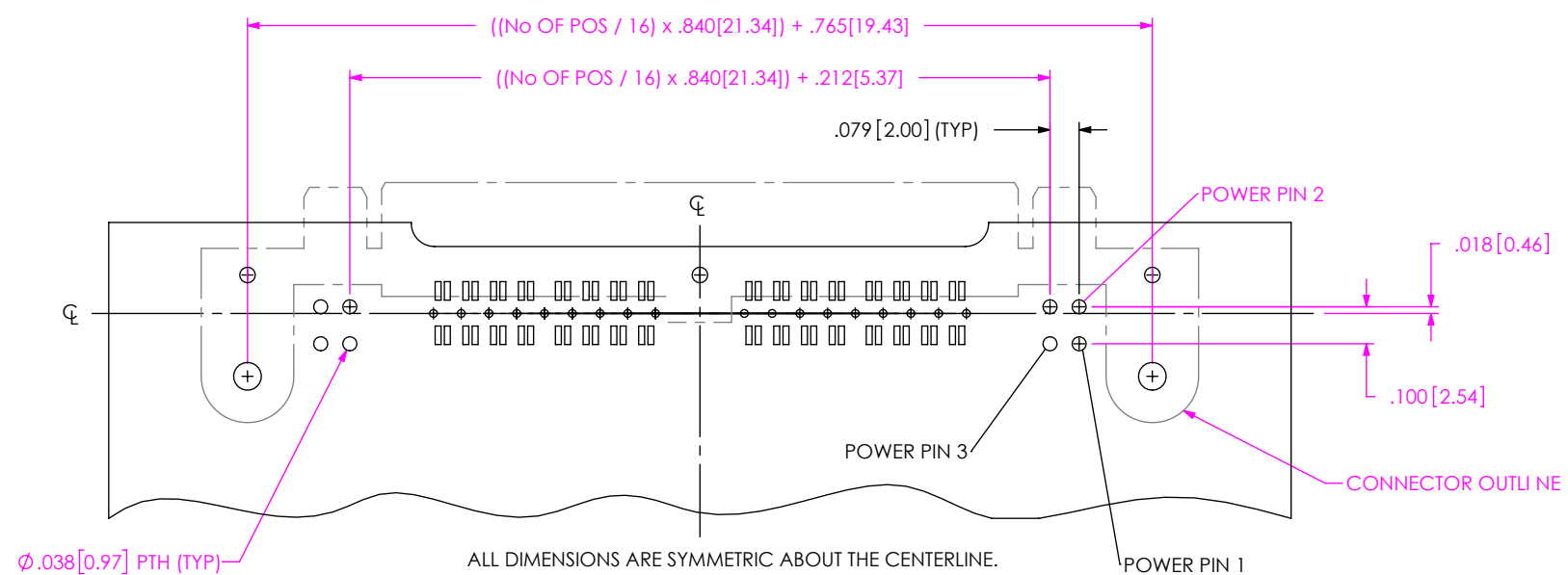
FIG 4 (QFS-032-01-XX-D-DP-RA-PC8 SHOWN) (DIFFERENT AS SHOWN, OTHERWISE SAME AS FIG 1)
