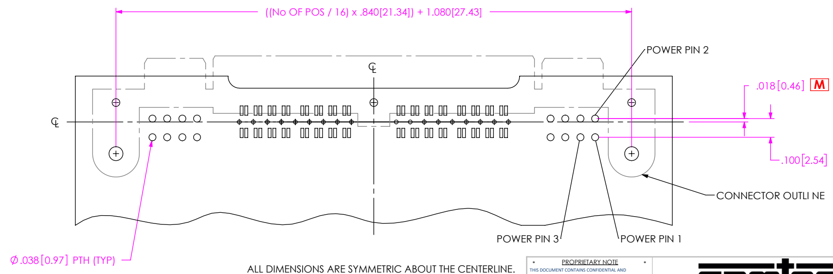
FIG 4 (QFS-032-01-XX-D-DP-RA-PC8 SHOWN) (DIFFERENT AS SHOWN, OTHERWISE SAME AS FIG 1)
