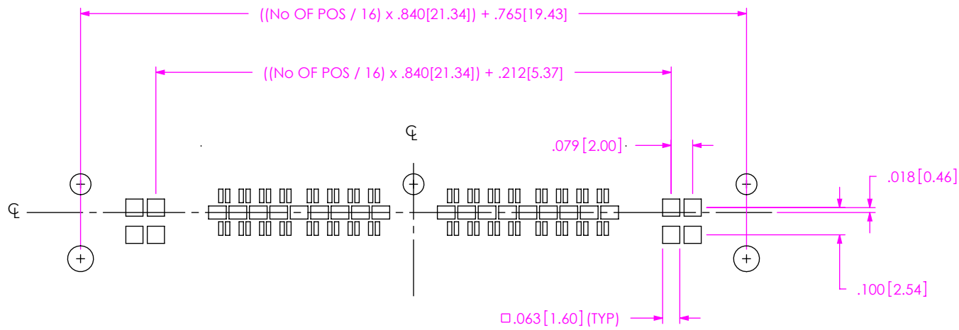
FIG 5 (QFS-032-01-XX-D-DP-RA-PC4 SHOWN) (DIFFERENT AS SHOWN, OTHERWISE SAME AS FIG 2)
