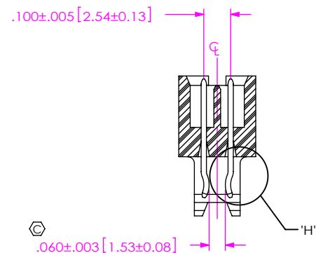
SECTION "G"-"G" SCALE 2 : 1
