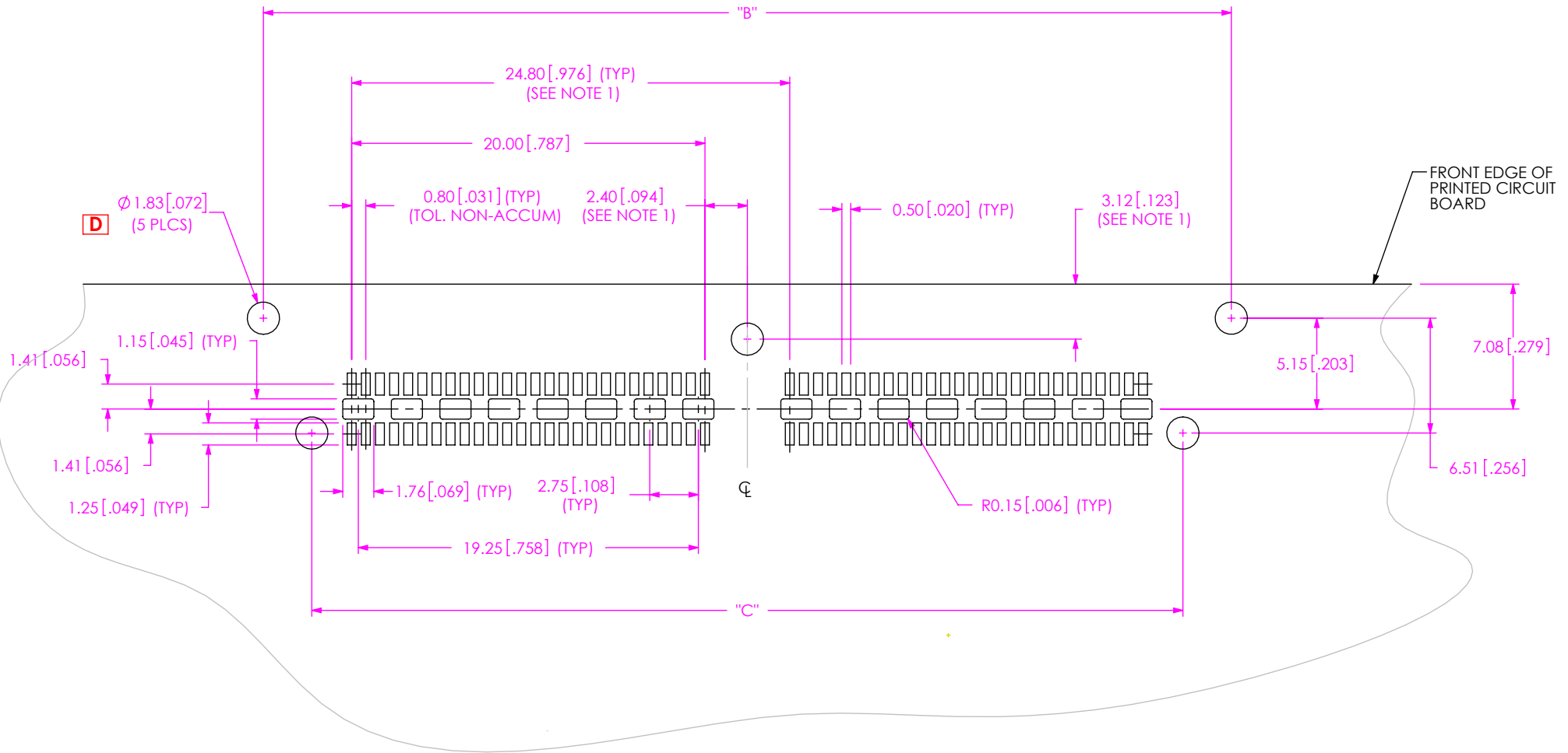
QRF8-052-XX-X-RA-GP (QRF8-052-02-X-RA-GP SHOWN) (ALL DIMENSIONS ARE SYMMETRIC ABOUT THE CENTERLINE)
