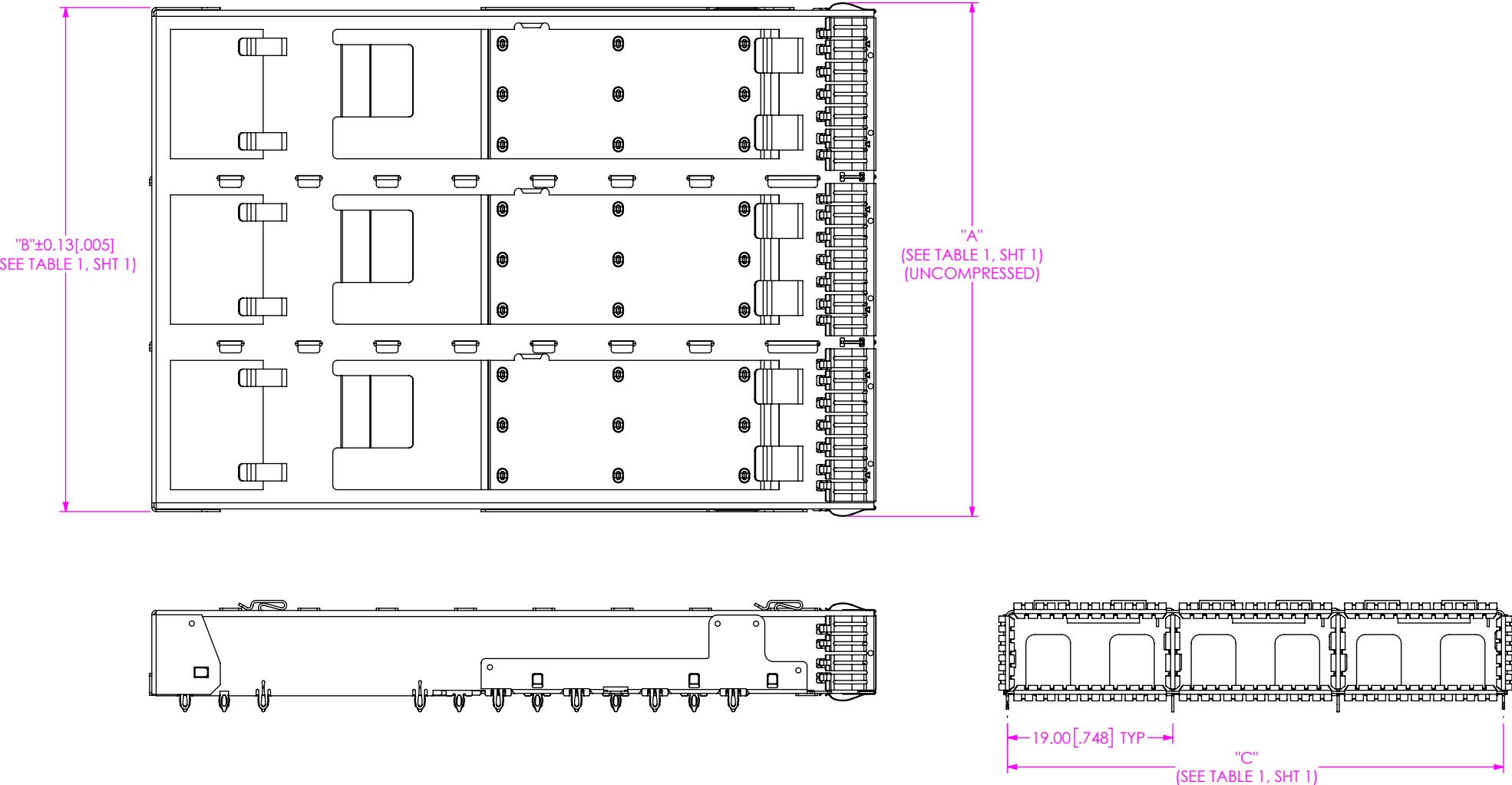
FIG 3 QSPFC-D8-R-1-3-S-F SHOWN (DIFFERENT AS SHOWN, OTHERWISE SAME AS FIG 1)
