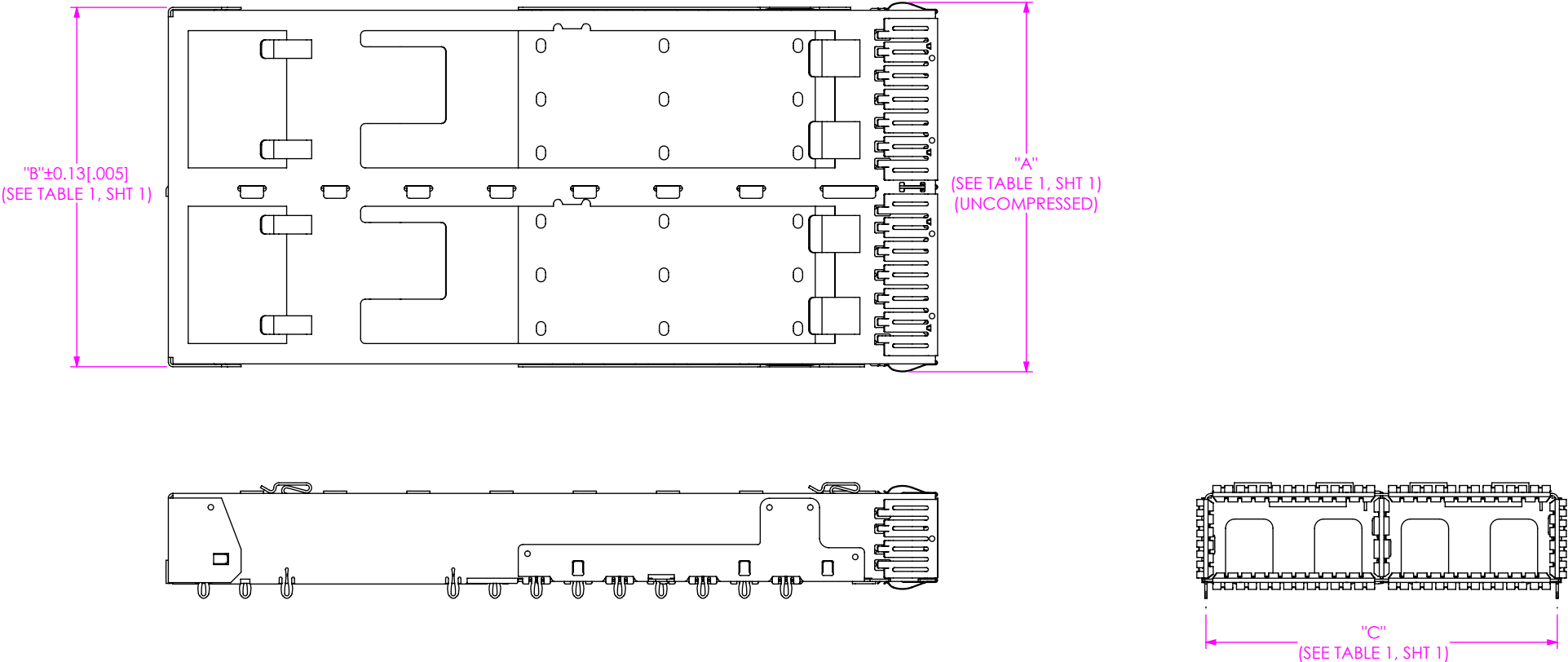
FIG 2 QSPFC-D8-R-1-2-S-F SHOWN (DIFFERENT AS SHOWN, OTHERWISE SAME AS FIG 1)
