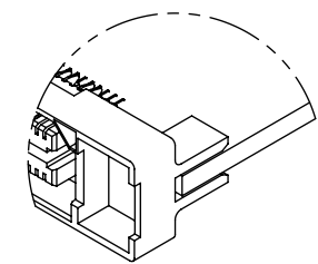
DETAIL WITH CONNECTOR SCALE 2:1
