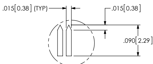
DETAIL "C" SCALE 3:1
