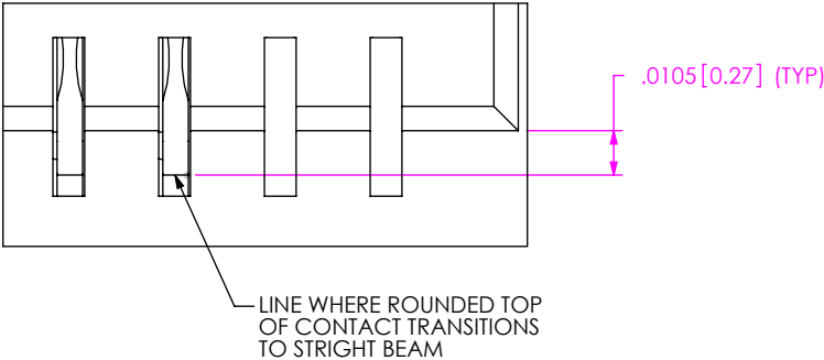
DETAIL 'A' SCALE 20: 1
