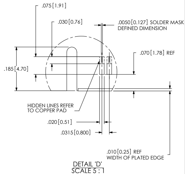
FIG 1: RECOMMENDED PCB LAYOUT FOR -DP OPTION
