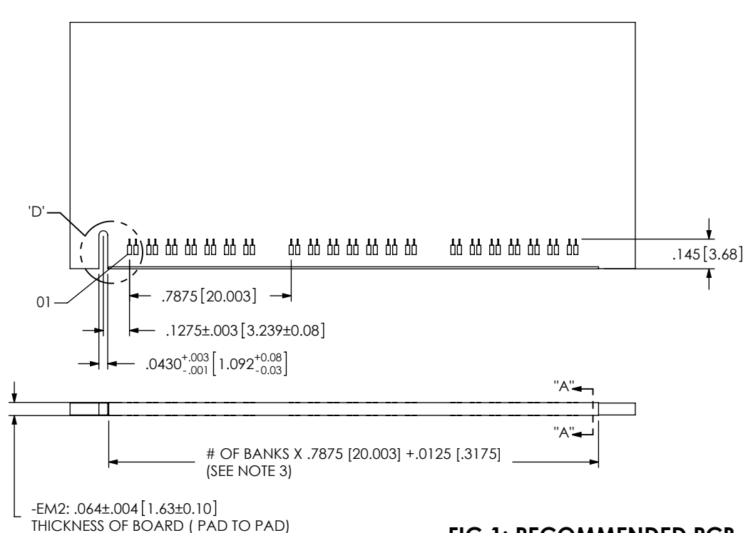
FIG 1: RECOMMENDED PCB LAYOUT FOR -DP OPTION
