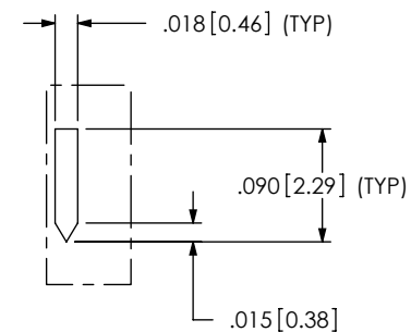
DETAIL 'C' SCALE 6:1
