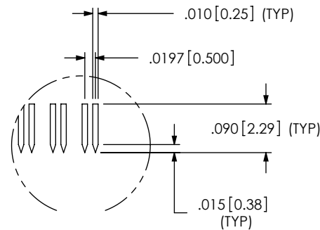
DETAIL 'C' SCALE 4 : 1
