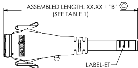
FIG 2 RC5-10-XX-X-D-XX.XX-BC SHOWN (SAME AS FIG. 1, EXCEPT AS SHOWN)
