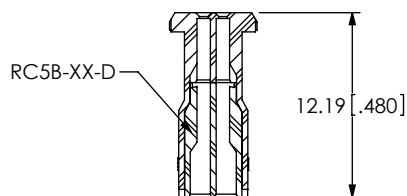
SECTION "D"-"D" SCALE 2 : 1
