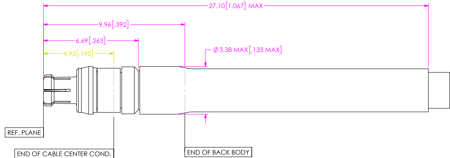
FIG 16 -GC86 SHOWN (COMPATIBLE WITH GC86 GANGED ASSEMBLY)
