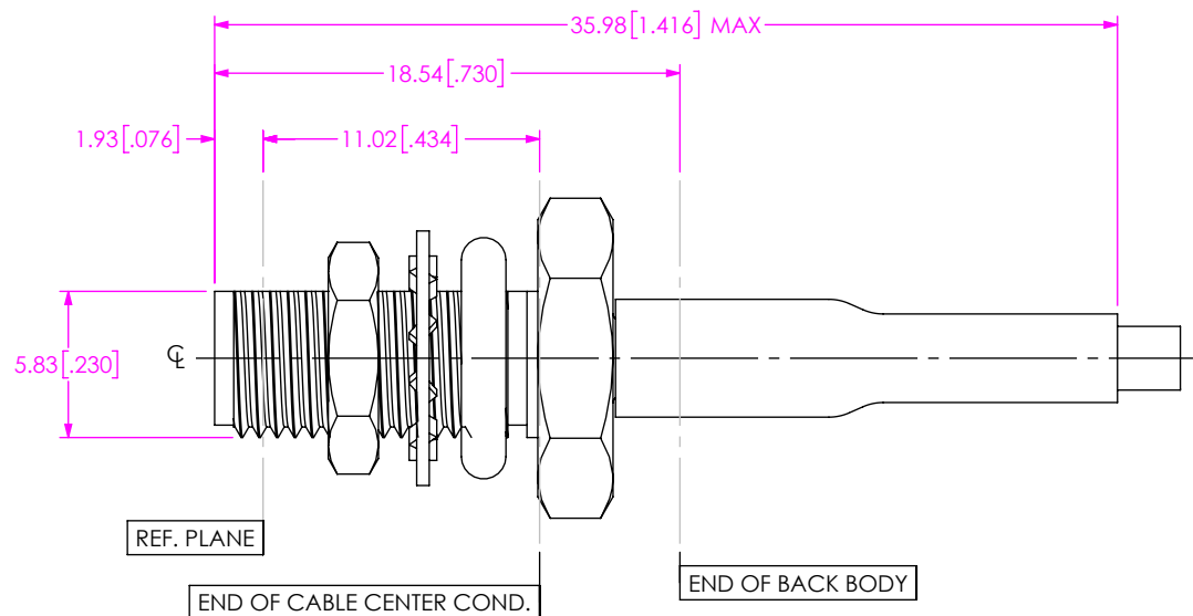
FIG 13 -01SB SHOWN (PROTECTIVE CAP NOT SHOWN FOR CLARITY)
