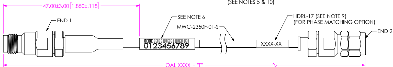
FIG 1 RF086-24SJ-18SP-XXXX-X-XX SHOWN (PROTECTIVE CAPS NOT SHOWN FOR CLARITY)
