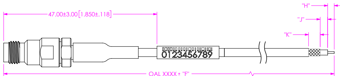
FIG 8 RF086-24SJ-102030-XXXX SHOWN (SEE NOTE 7 & 8)
