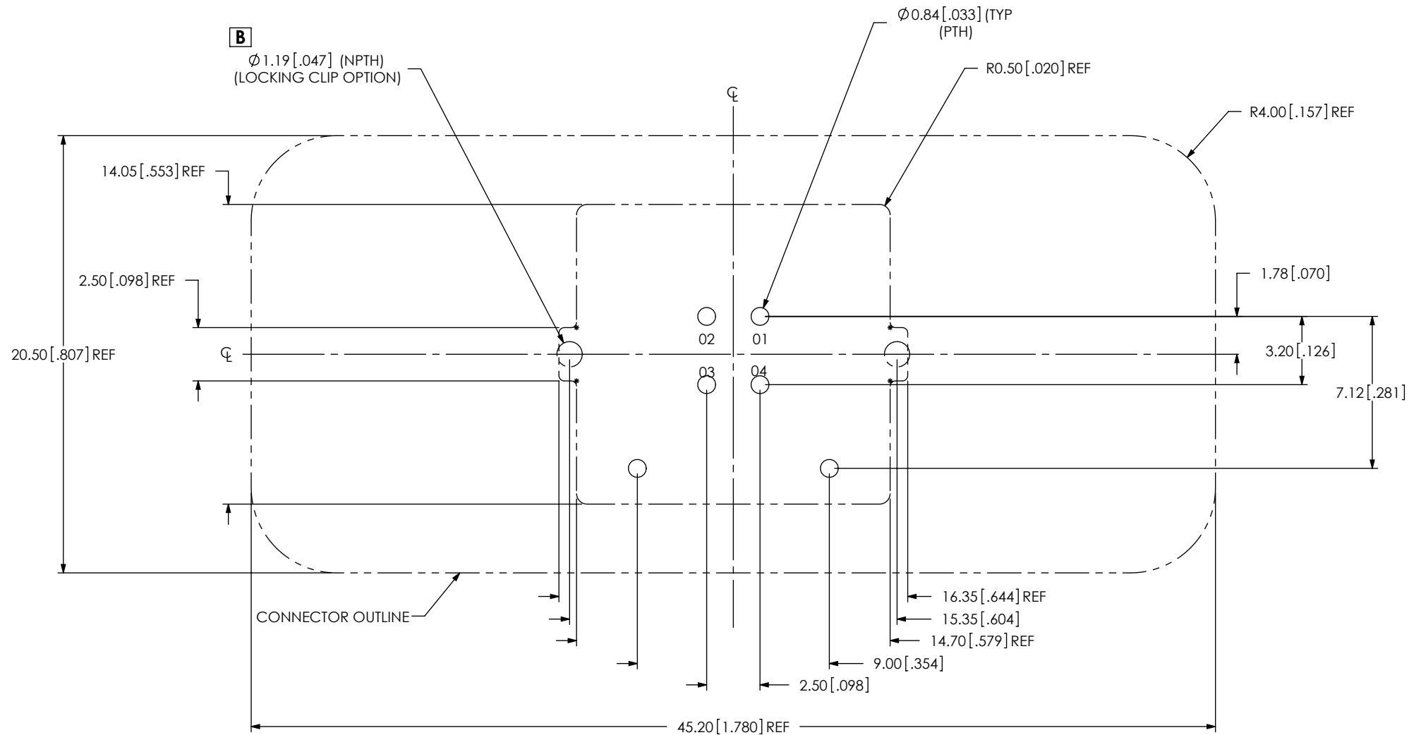
FIG 2 RPBU-01-X-B-VT-XX SHOWN ALL DIMENSIONS ARE SYMMETRIC ABOUT THE CENTERLINE.
