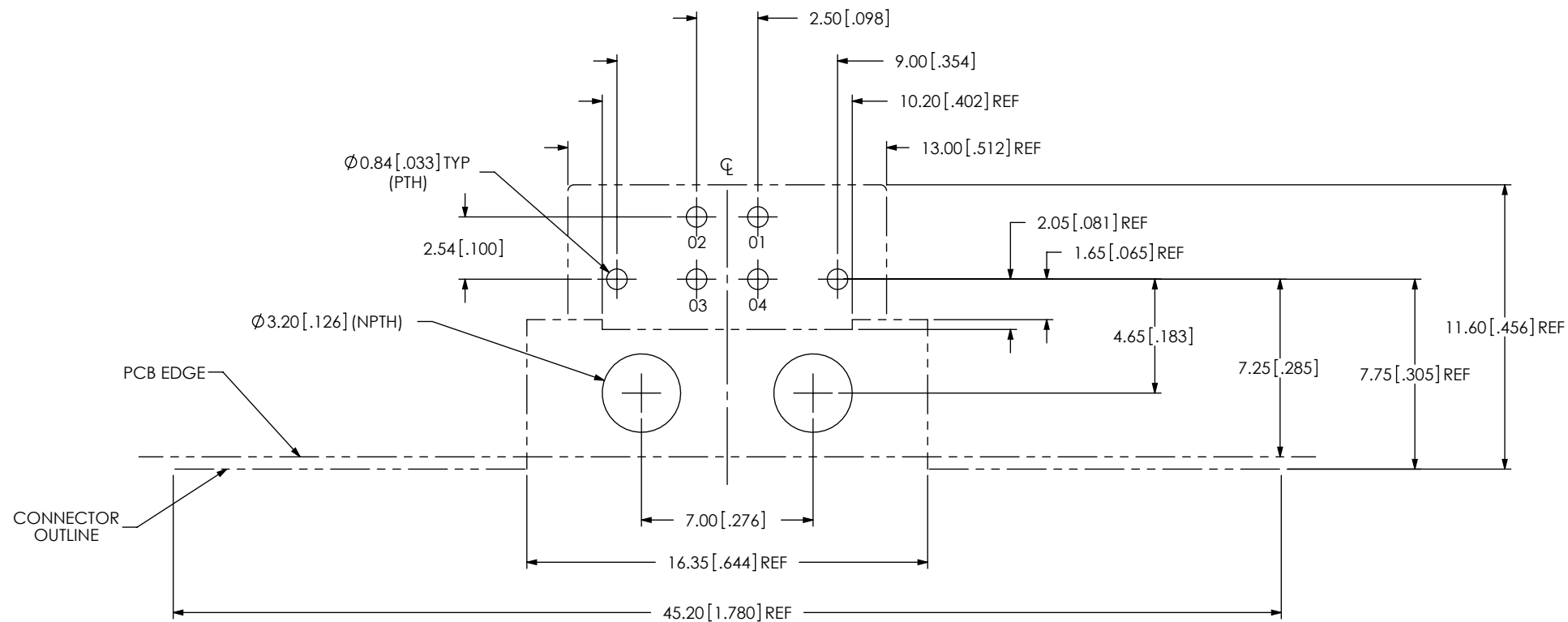
FIG 1 RPBU-01-X-B-RA SHOWN ALL DIMENSIONS ARE SYMMETRIC ABOUT THE CENTERLINE.
