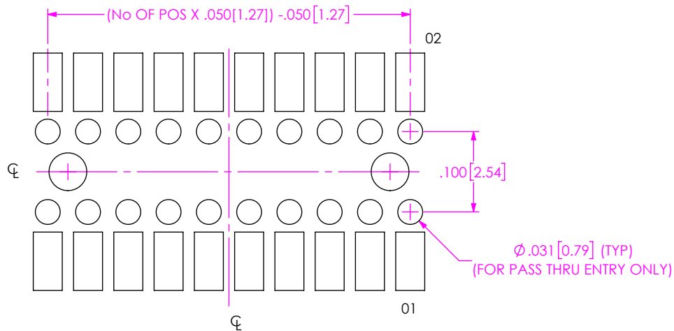
FIG 2 (FOR PASS THRU ENTRY) RSM-110-XX-XXX-D-XX-FOOTPRINT SHOWN (DIFFERENT AS SHOWN, OTHERWISE SAME AS FIG 1)
