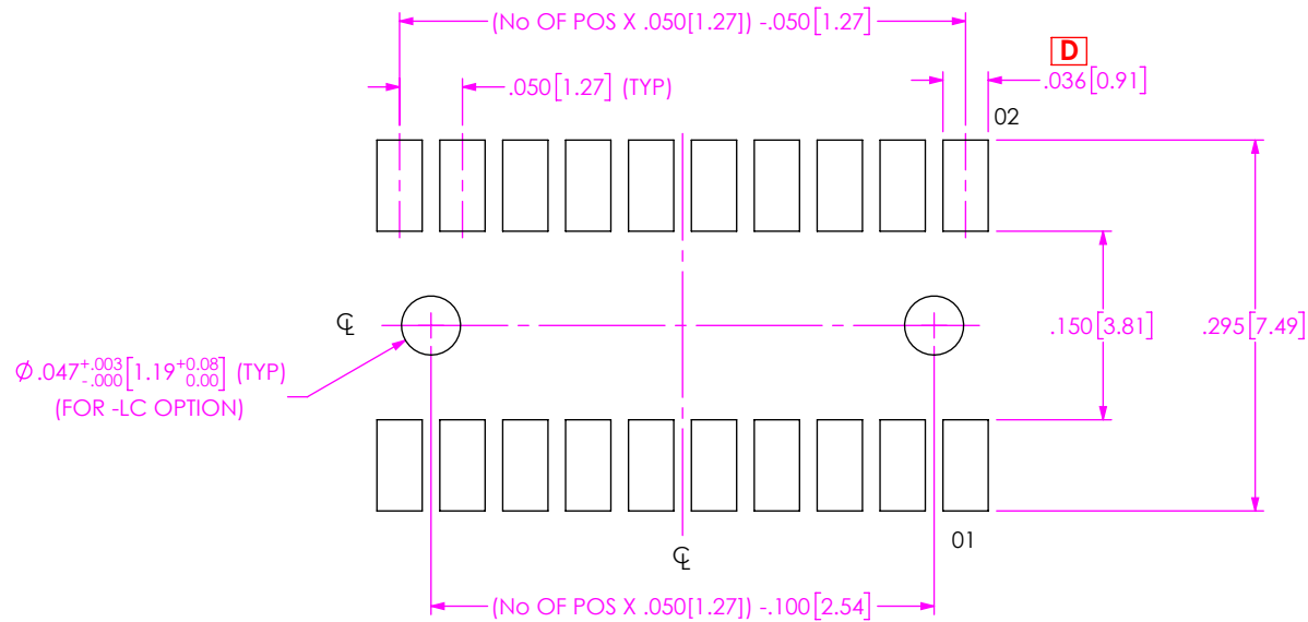
FIG 1 RSM-110-XX-XXX-D-XX-FOOTPRINT SHOWN
