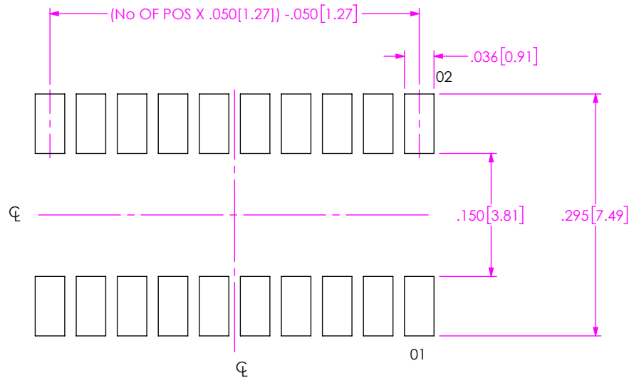
FIG 3 D RSM-110-XX-XXX-D-XX-STENCIL SHOWN
