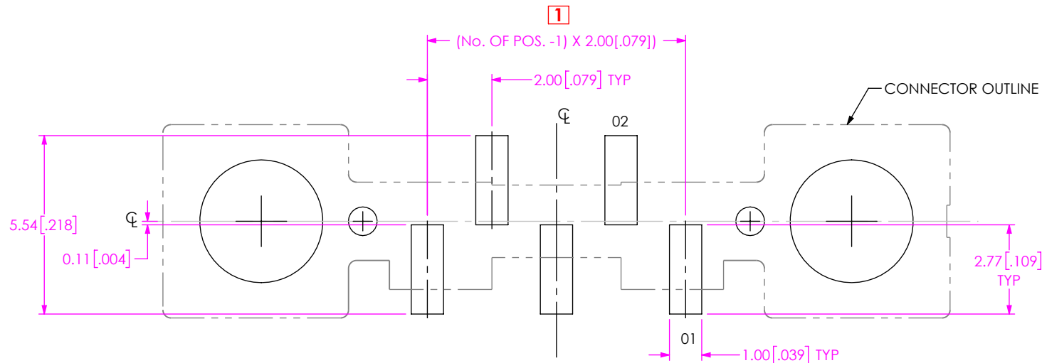
FIG 3 S2M-105-01-X-S-DS SHOWN (SAME AS FIG 1, EXPECT AS SHOWN)
