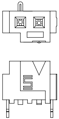
FIG 3 S2M-102-02-X-S-LC SHOWN (SAME AS FIG 2, EXCEPT AS SHOWN)
