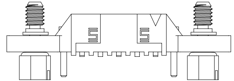
FIG 5 S2M-105-02-X-S-DS SHOWN (SAME AS FIG 4, EXCEPT AS SHOWN)
