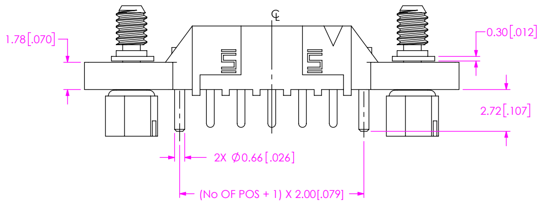
FIG 4 S2M-105-01-X-S-DS SHOWN (SAME AS FIG 1, EXCEPT AS SHOWN)
