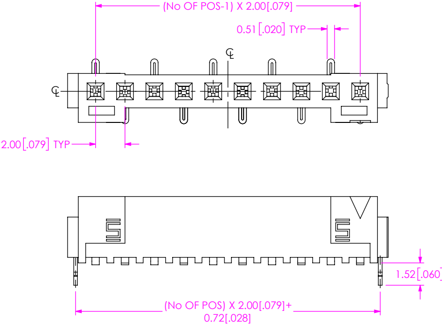
FIG 2 S2M-110-02-X-S-LC SHOWN (SAME AS FIG 1, EXCEPT AS SHOWN)
