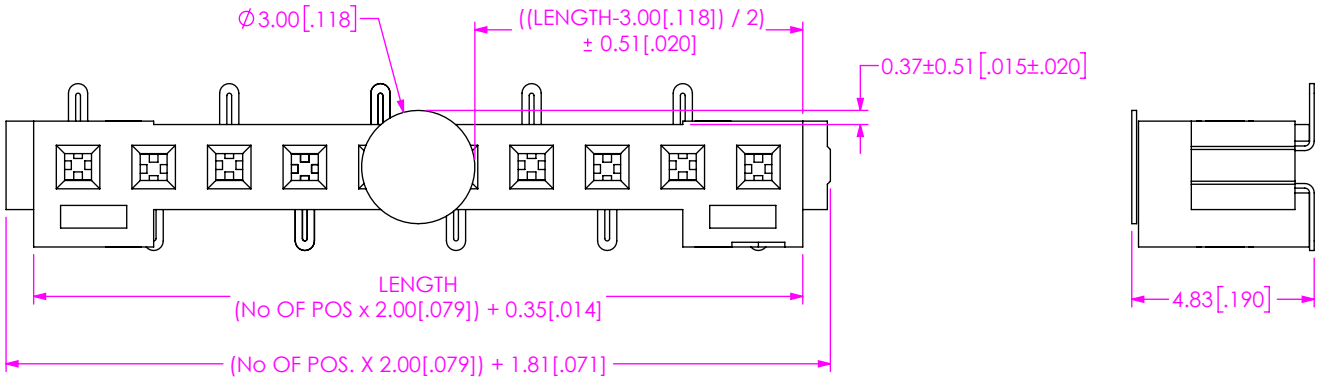
FIG 6 S2M-110-02-X-S-K SHOWN (SAME AS FIG 2, EXCEPT AS SHOWN)
