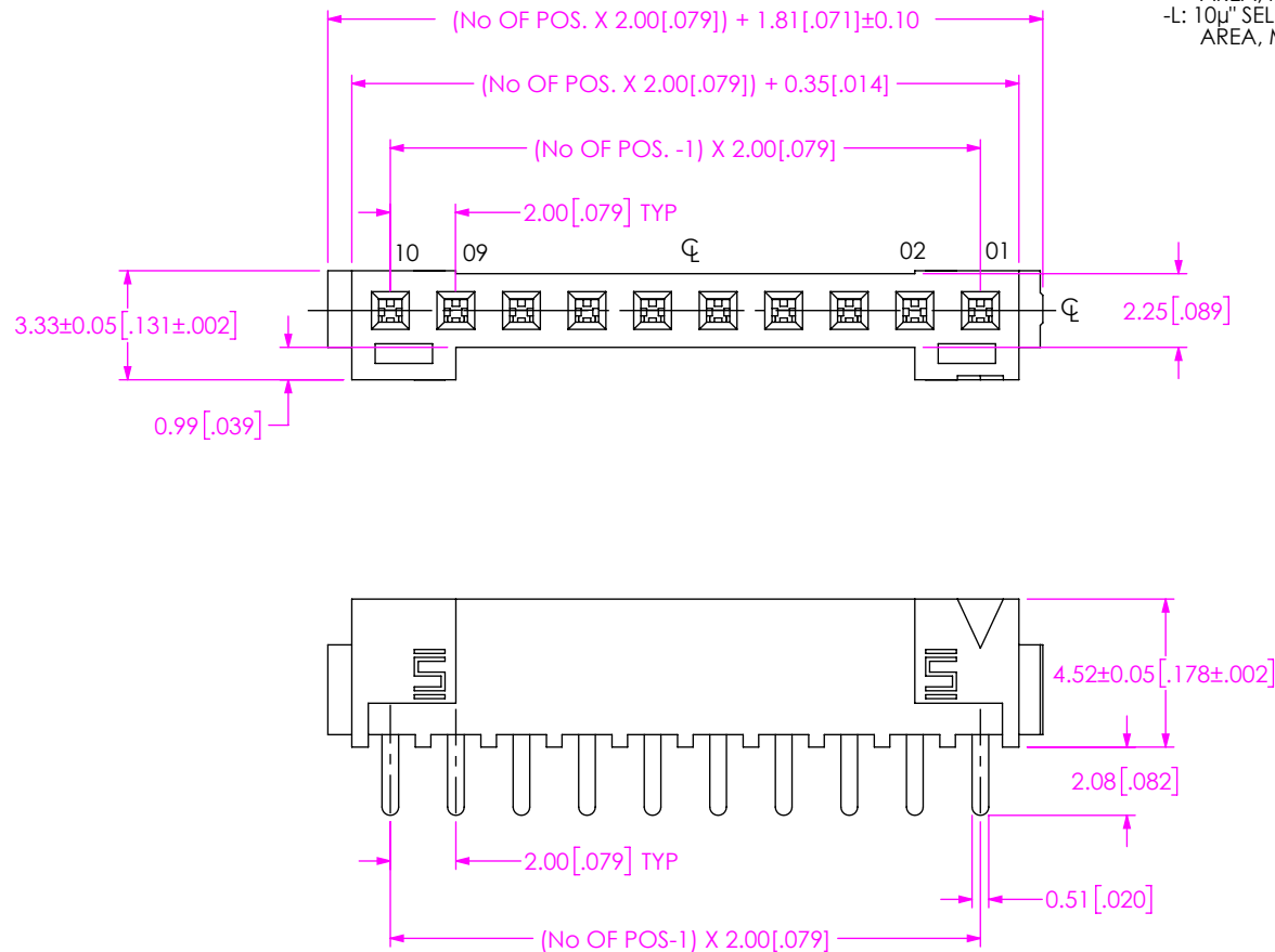
FIG 1 S2M-110-01-XX-S SHOWN
