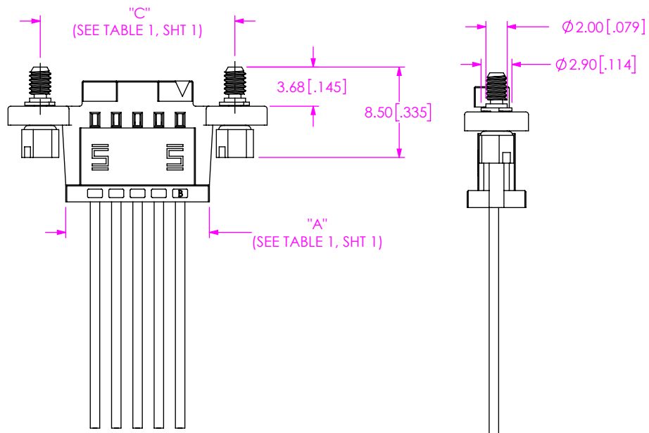
FIG 7 -SS: SINGLE ENDED WITH SCREW DOWN (S2SSX-05-28-X-XX.XX-SS SHOWN) (SAME AS FIG 1, EXCEPT AS SHOWN)
