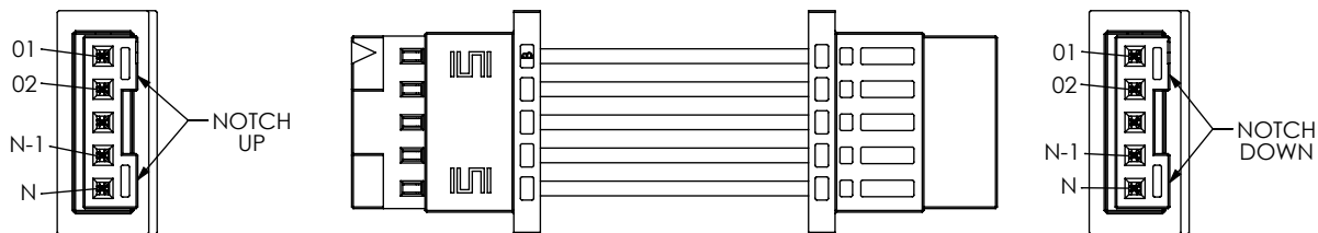
FIG 3 (S2SSX-05-28-X-XX.XX-D-NDS SHOWN) (SAME AS FIG 1, EXCEPT AS SHOWN) (PIN 01 TO 01)
