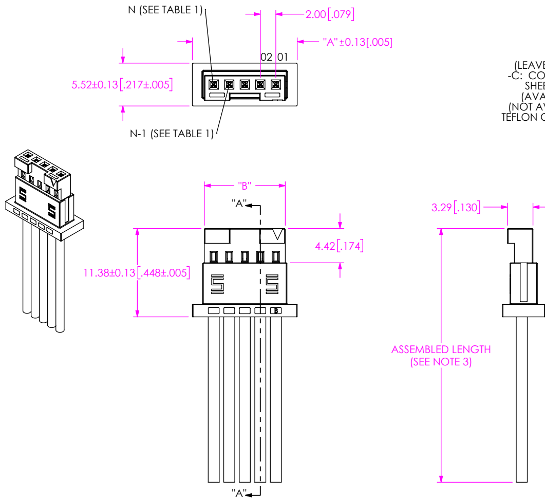
FIG 1 S2SSX-05-24-X-XX.XX-S SHOWN
