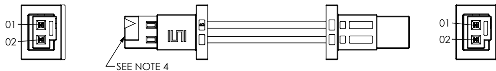
FIG 4 (S2SSX-02-28-X-XX.XX-D-NDS SHOWN) (SAME AS FIG 3, EXCEPT AS SHOWN) (PIN 01 TO 01)
