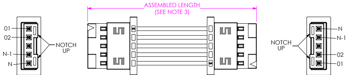
FIG 2 (S2SSX-05-28-X-XX.XX-D-NUS SHOWN) (SAME AS FIG 1, EXCEPT AS SHOWN) (PIN 01 TO N)
