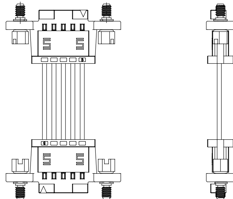
FIG 8 -DS: DOUBLE ENDED WITH SCREW DOWN (S2SSX-05-28-X-XX.XX-DS-NUS SHOWN) (SAME AS FIG 7, EXCEPT AS SHOWN)
