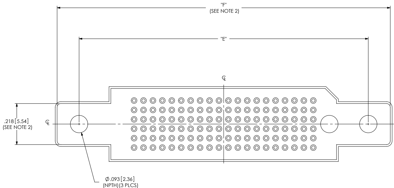
FIG 2 (GUIDE POST OPTION) (SEAMP-20-02.0-X-06-GP1 FOOTPRINT SHOWN) (SAME AS FIG 1 EXCEPT AS SHOWN)
