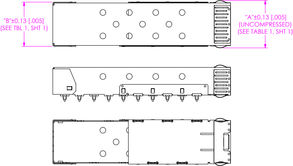
FIG 8 SFPC-1-1-S-H-F SHOWN (DIFFERENT AS SHOWN, OTHERWISE SAME AS FIG 6)
