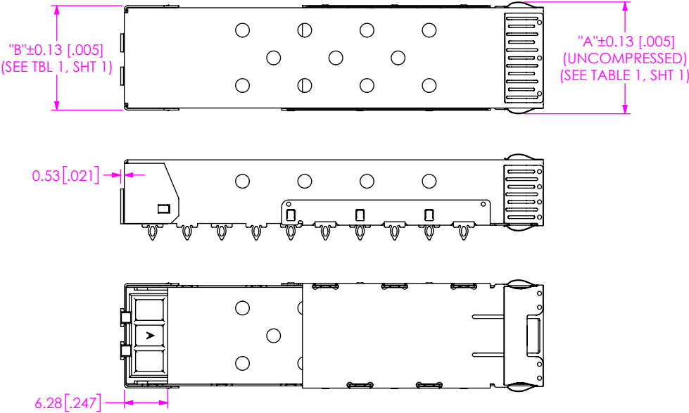
FIG 10 SFPC-1-1-S-A-F SHOWN (DIFFERENT AS SHOWN, OTHERWISE SAME AS FIG 6)
