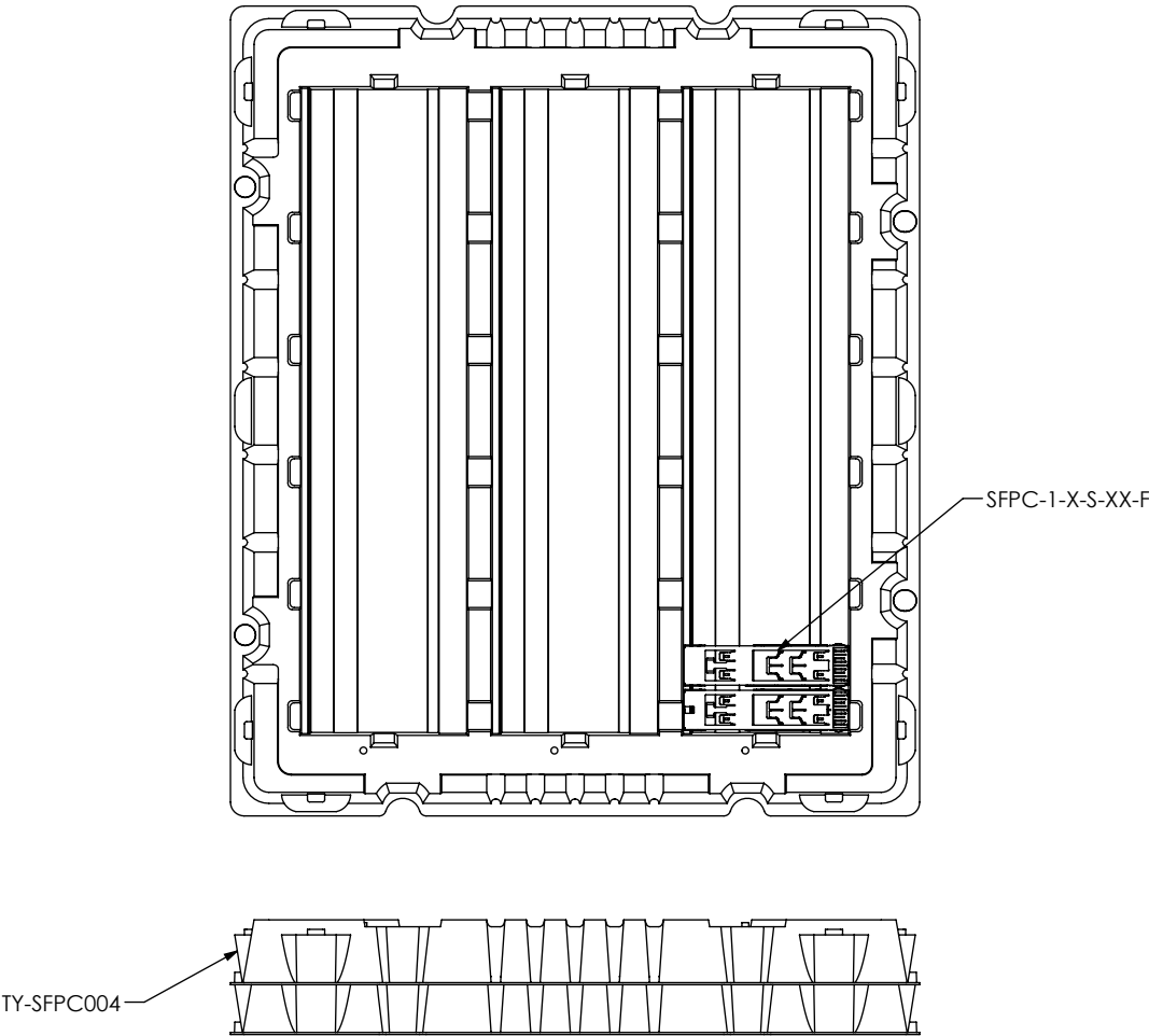
FIG 7 PACKAGING VIEW
