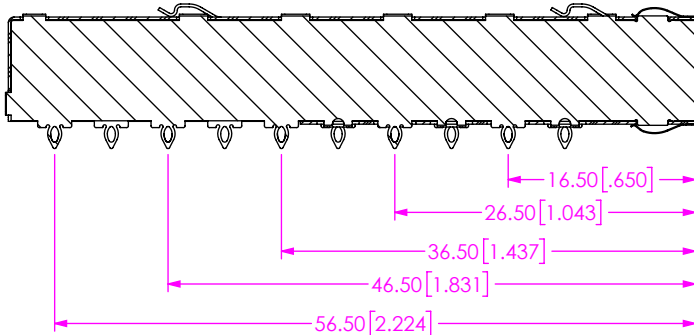
SECTION "B"- "B" SCALE 1.5 : 1
