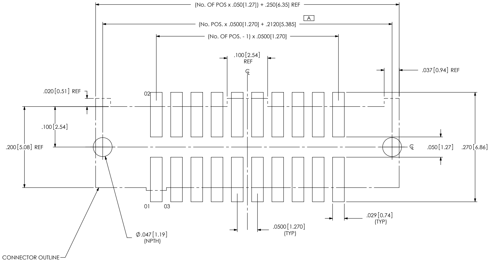
FIG. 1 (SHF-110-01-X-D-SM-LC SHOWN)
