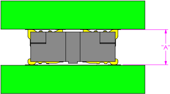
FIG 1 SLH-D MATED WITH TLH-D
