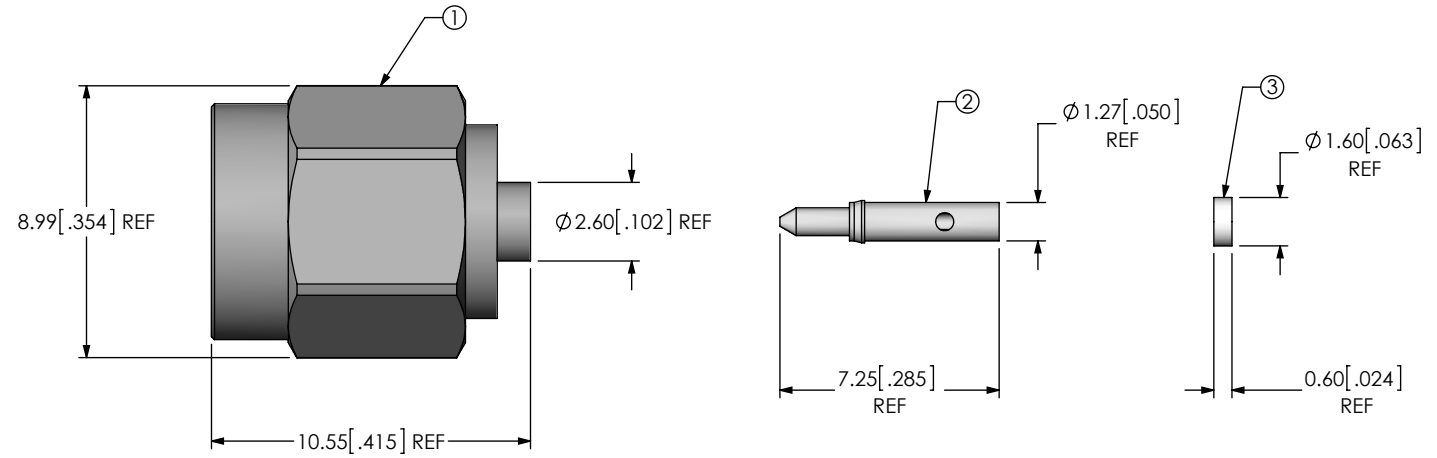
FIG 1 SMA-P-C-X-ST-CA5 SHOWN
