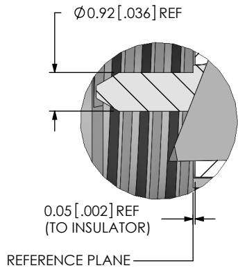
DETAIL 'A' SCALE 8:1
