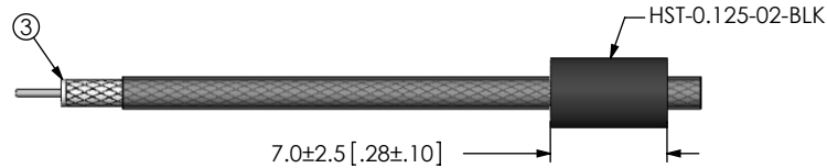
IN-PROCESS 3 ADD INSULATOR AND HEAT SHRINK TUBE
