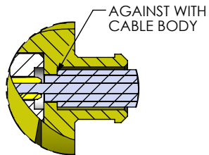
DETAIL 'C' SCALE 6:1
