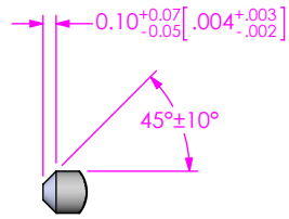
DETAIL 'B' SCALE 16:1
