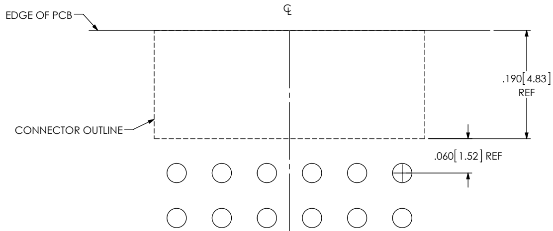
B FIG 2 STMM-1XX-XX-XX-D-RA SHOWN SAME AS FIG 1, EXCEPT AS SHOWN
