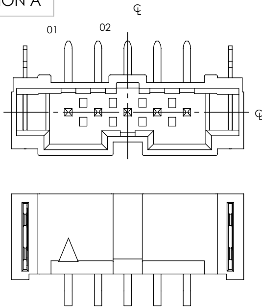
FIG 2 T2M-105-01-X-S-RA-XX (SAME AS FIG 1, EXCEPT AS SHOWN)
