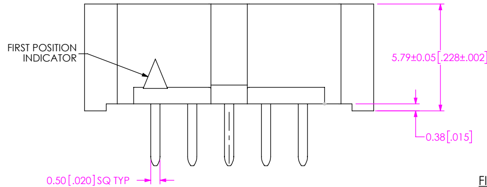
FIG 1 T2M-105-01-X-S-TH
