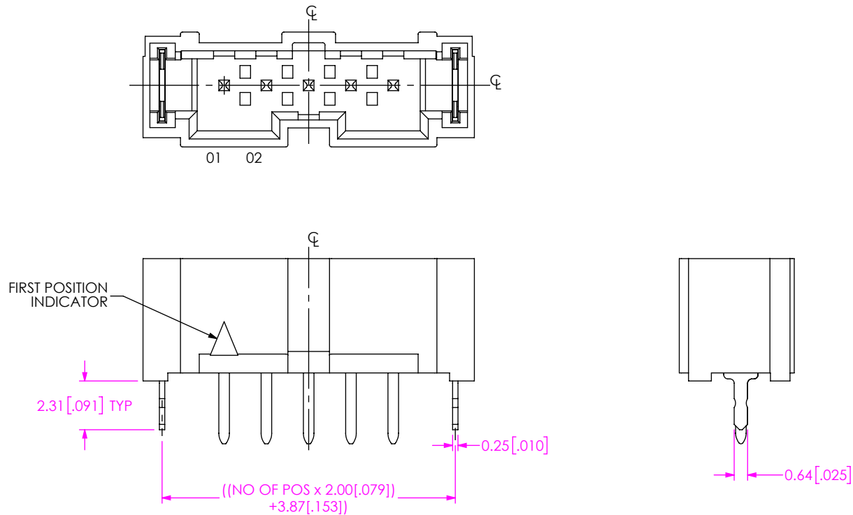
FIG 8 T2M-105-01-X-S-TH-WT SHOWN (SAME AS FIG 1, EXCEPT AS SHOWN)
