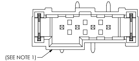
FIG 4 T2M-102-01-X-S-SM (SAME AS FIG 1, EXCEPT AS SHOWN)
