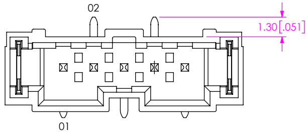
FIG 2 T2M-105-01-X-S-RA-XX (SAME AS FIG 1, EXCEPT AS SHOWN)
