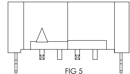
FIG 5 T2M-104-01-X-S-SM-WT (SAME AS FIG 1, EXCEPT AS SHOWN) (T2M-102-01-X-S-SM-WT SIMILAR)
