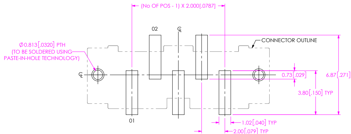
FIG 2 T2M-105-01-XX-S-SM-WT SHOWN (SAME AS FIG 1, EXCEPT AS SHOWN)
