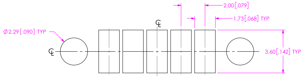
FIG 3 (T2M-105-01-XX-S-TH-WT SHOWN) (SAME AS FIG 1, EXCEPT AS SHOWN)
