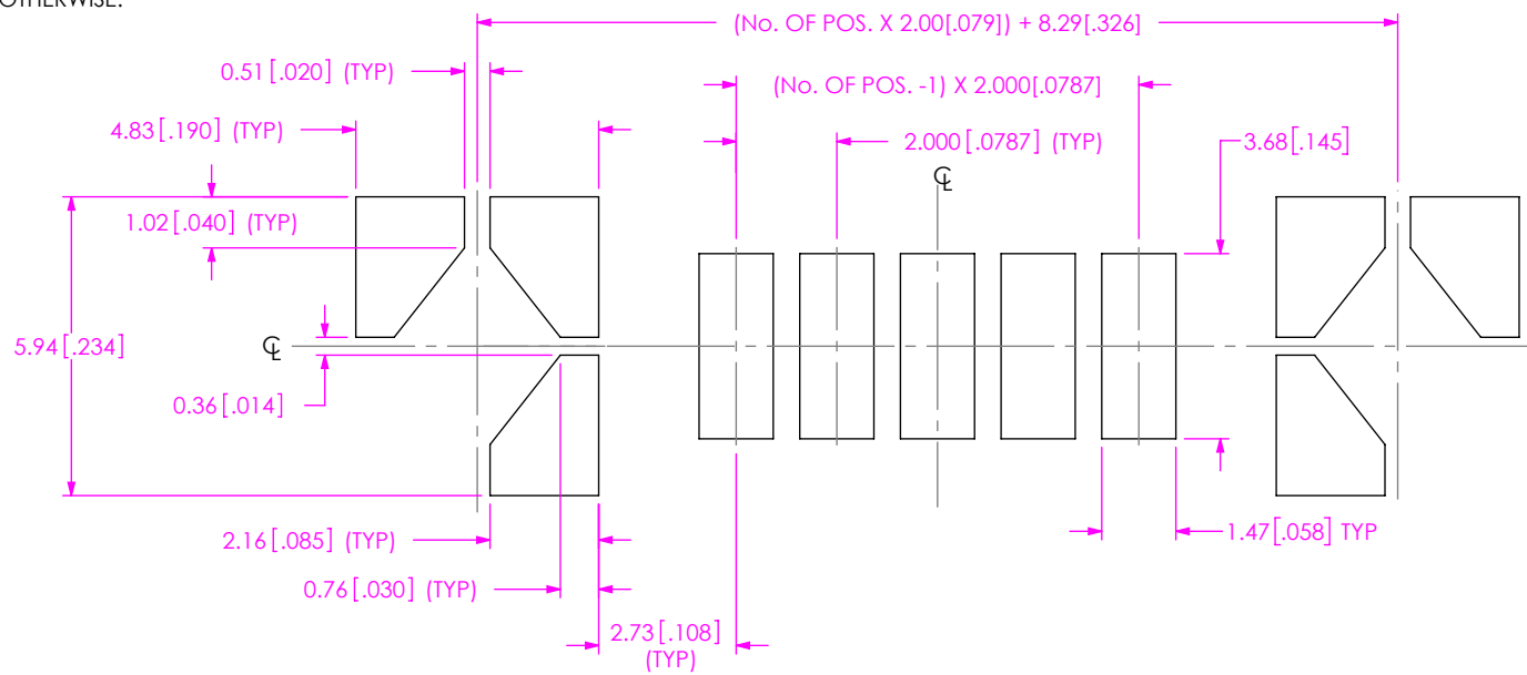
FIG 8 (T2M-105-01-XX-S-SM-DS SHOWN) (SAME AS FIG 7, EXCEPT AS SHOWN)
