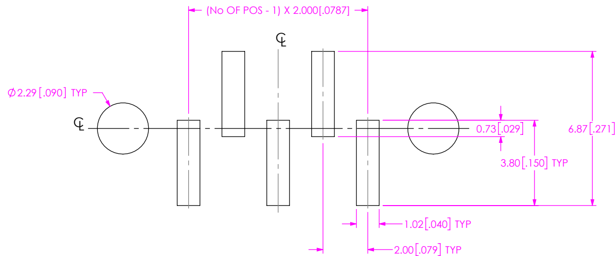
FIG 4 (T2M-105-01-XX-S-SM-WT SHOWN) (SAME AS FIG 1, EXCEPT AS SHOWN)
