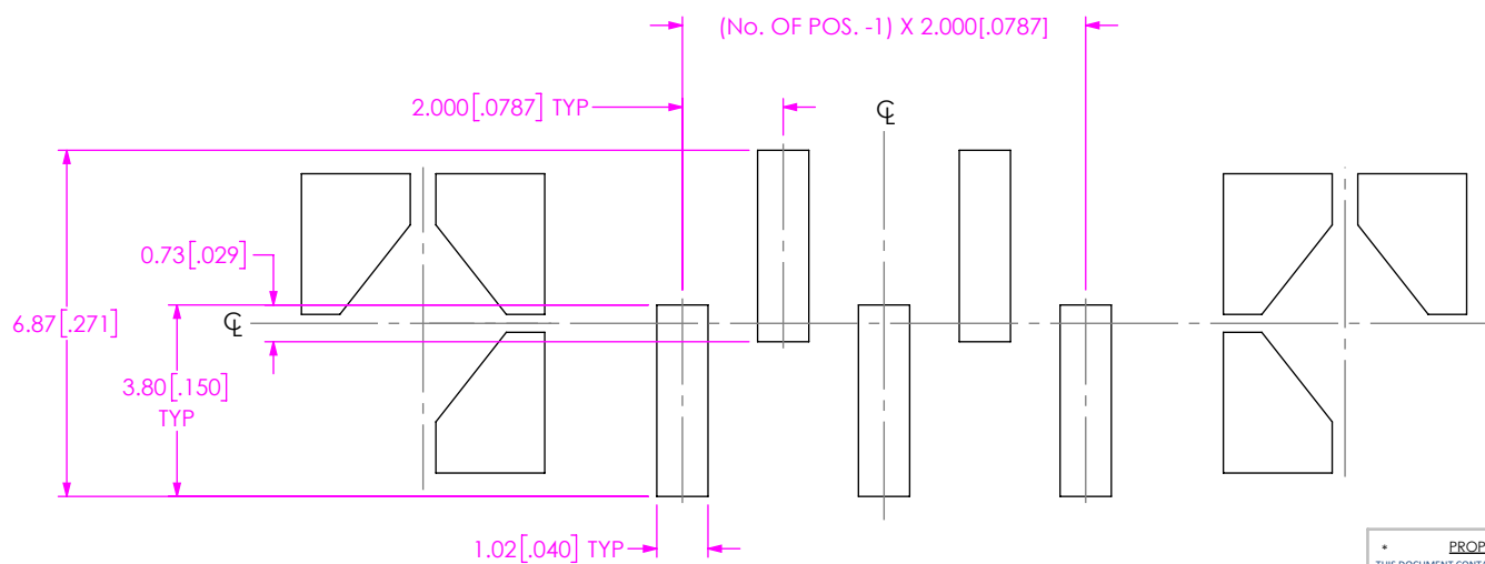
FIG 8 (T2M-105-01-XX-S-SM-DS SHOWN) (SAME AS FIG 7, EXCEPT AS SHOWN)
