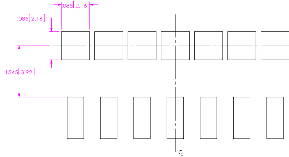
FIG 2 B TSM-MT SHOWN (DIFFERENT AS SHOWN, OTHERWISE SAME AS FIG 1) (ALL DIMENSIONS ARE SYMMETRIC ABOUT THE CENTERLINE)
