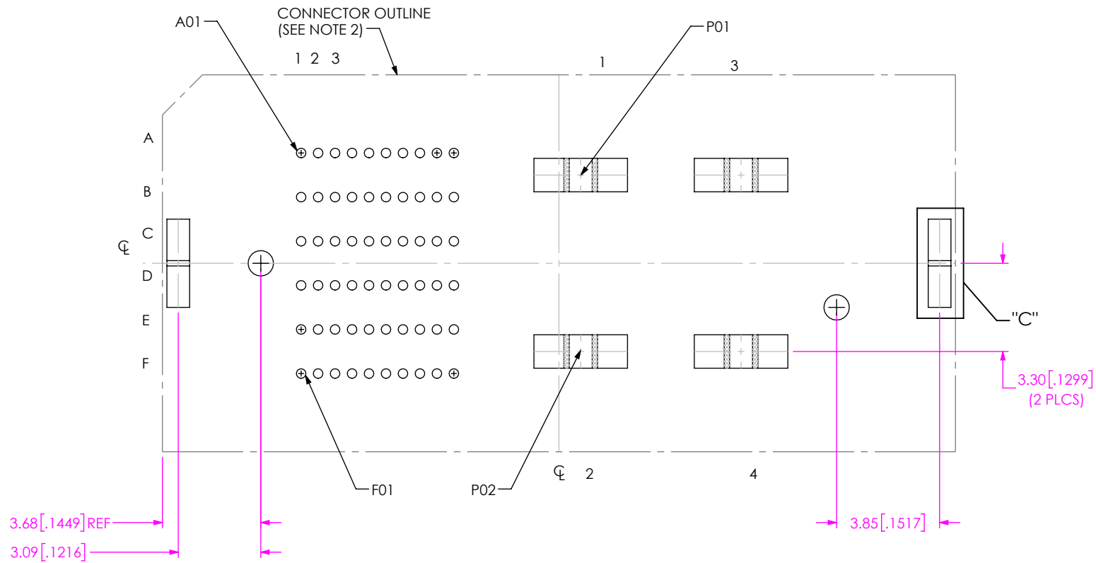
FIG 2 UDM6-10-2-XX.X-XXX-A-SM-XR SHOWN (DIFFERENT AS SHOWN, OTHERWISE SAME AS FIG 1)
