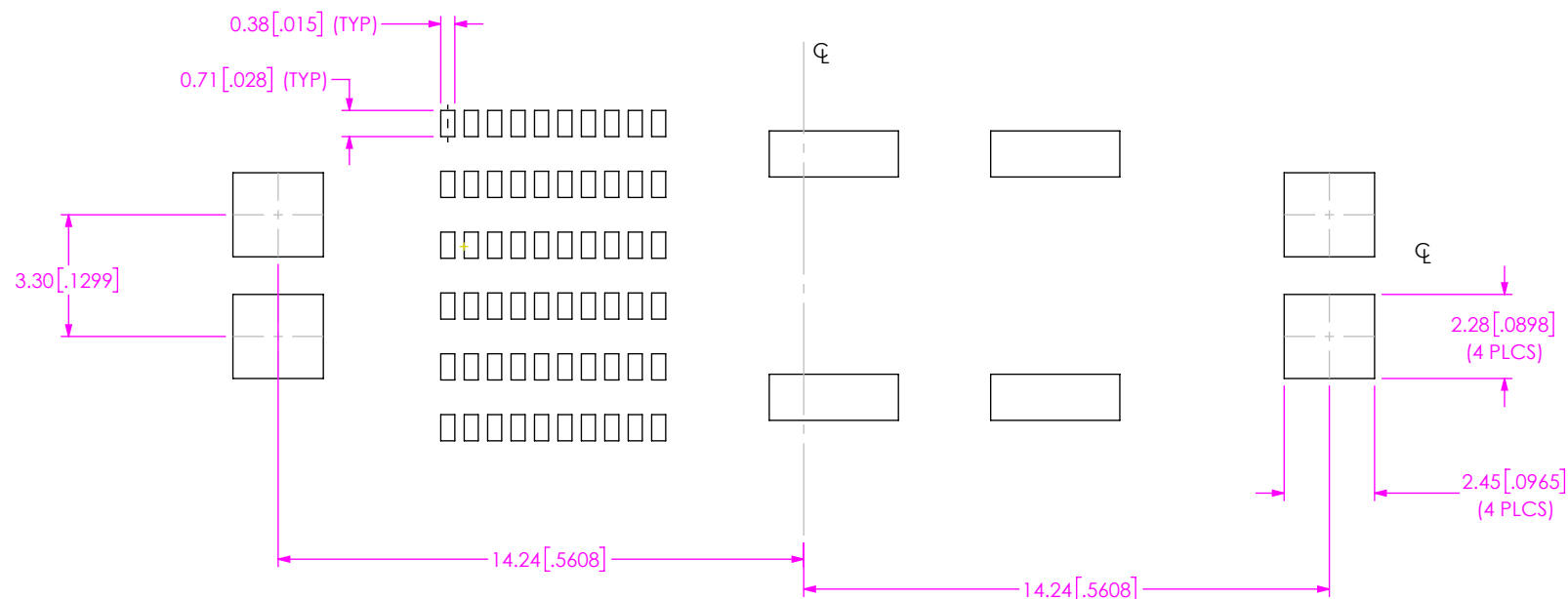
FIG 3 UDM6-10-2-XX.X-XXX-A-SM STENCIL SHOWN DIFFERENT AS SHOWN, OTHERWISE SAME AS FIG 1
