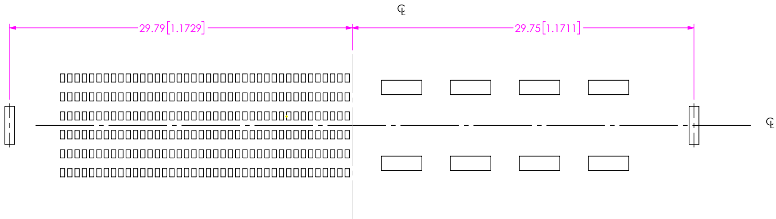
FIG 6 UDM6-40-4-XX.X-XXX-A-SM STENCIL SHOWN DIFFERENT AS SHOWN, OTHERWISE SAME AS FIG 4
