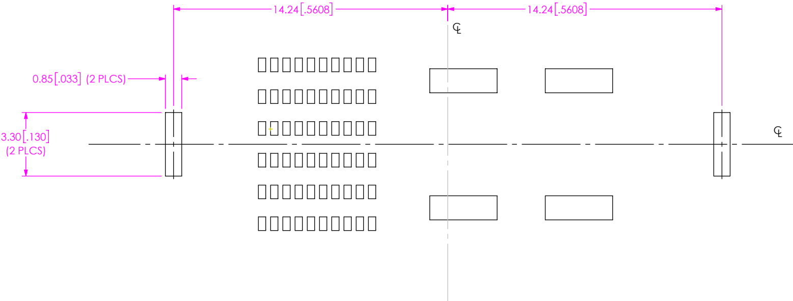
FIG 4 UDM6-10-2-XX.X-XXX-A-SM STENCIL SHOWN DIFFERENT AS SHOWN, OTHERWISE SAME AS FIG 2
