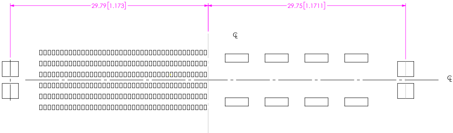
FIG 5 UDM6-40-4-XX.X-XXX-A-TH STENCIL SHOWN DIFFERENT AS SHOWN, OTHERWISE SAME AS FIG 3
