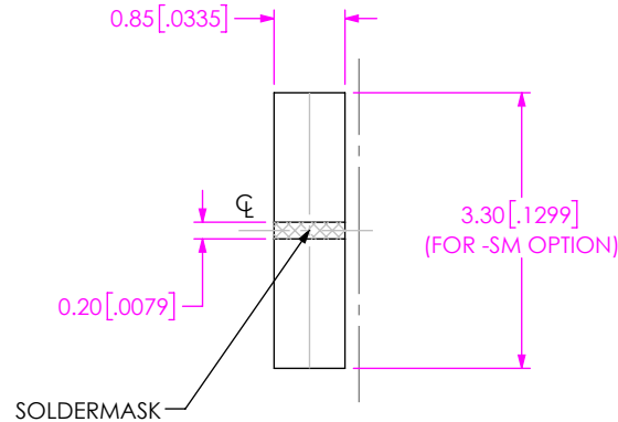
DETAIL "C" SCALE 10:1
