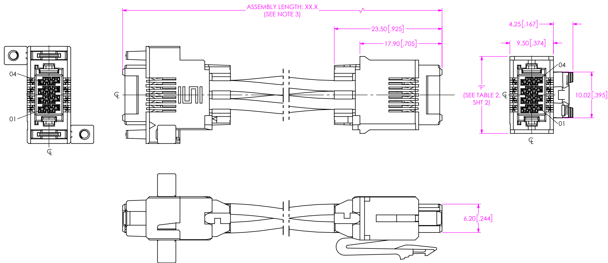
FIG 3 UMPIX-04-X-XX-XX.X-P1 SHOWN (DIFFERENT AS SHOWN, OTHERWISE SAME AS FIG 1)
