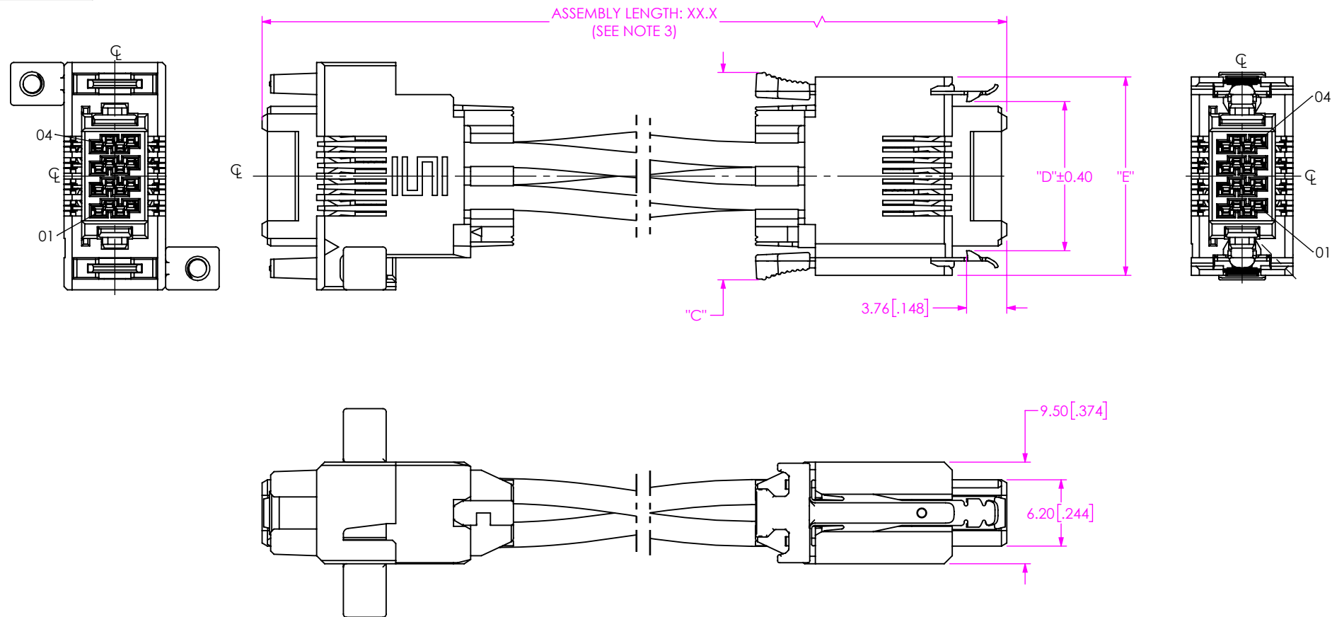
FIG 2 UMPIX-04-X-XX-XX.X-M1 SHOWN (DIFFERENT AS SHOWN, OTHERWISE SAME AS FIG 1)
