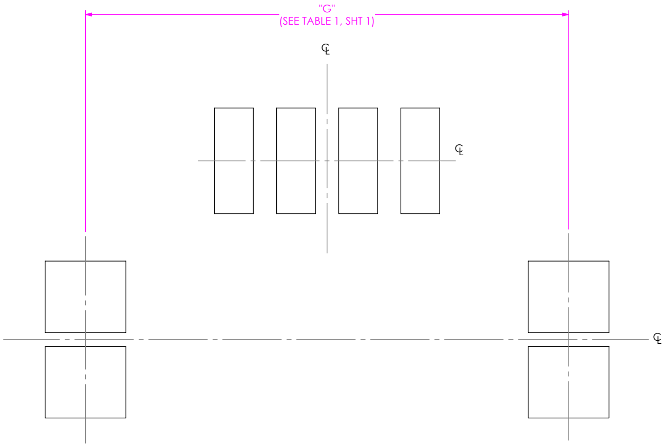
FIG 6 UMPT-04-01-XX-RA-X-WT-M STENCIL SHOWN (DIFFERENT AS SHOWN, OTHERWISE SAME AS FIG 1 & 2)
