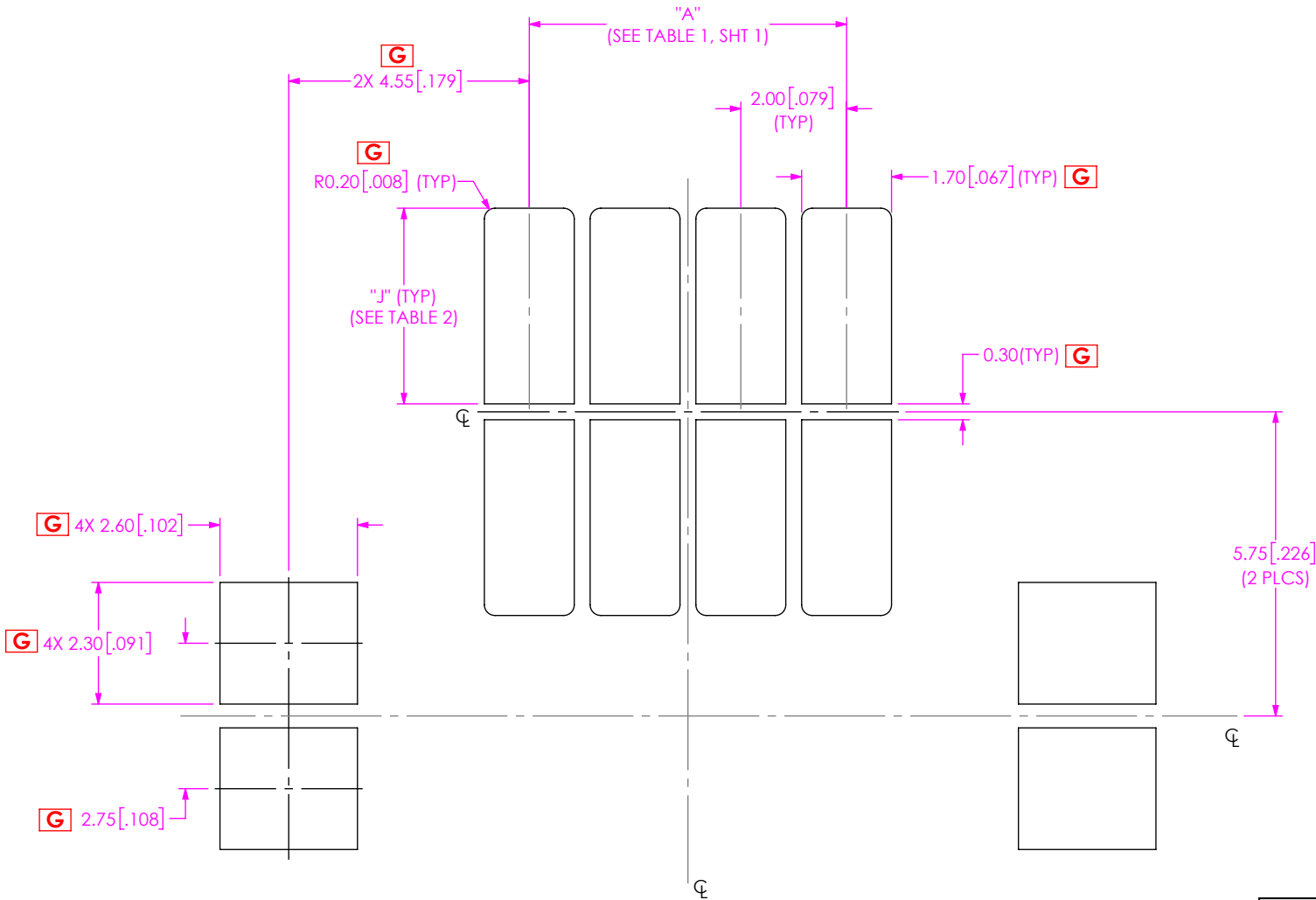
FIG 8 UMPT-04-XX-XX-RA-X-WT STENCIL SHOWN
