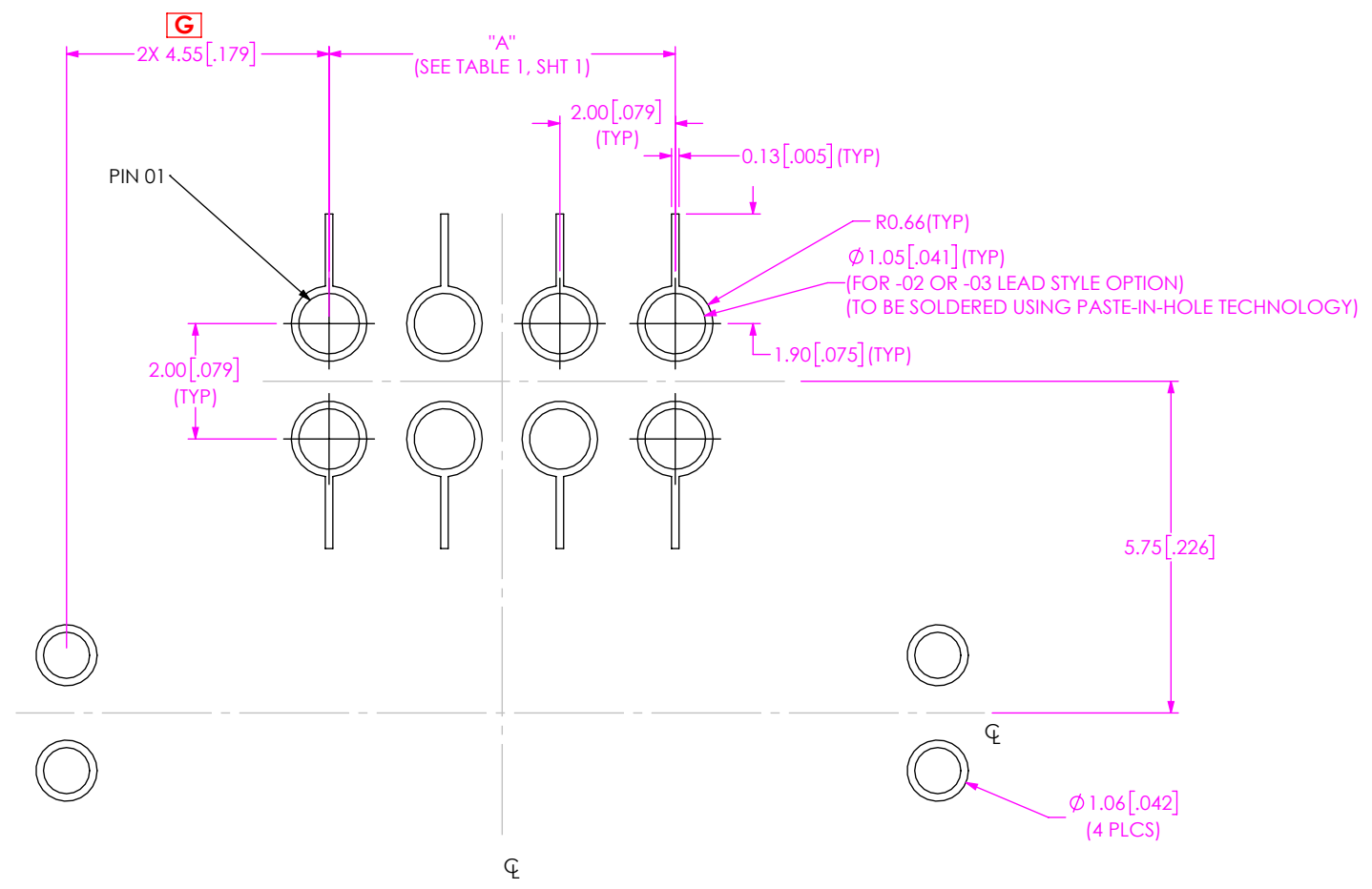
FIG 7 UMPT-04-XX-XX-RA-X-WT FOOTPRINT SHOWN (DIFFERENT AS SHOWN, OTHERWISE SAME AS FIG 1)
