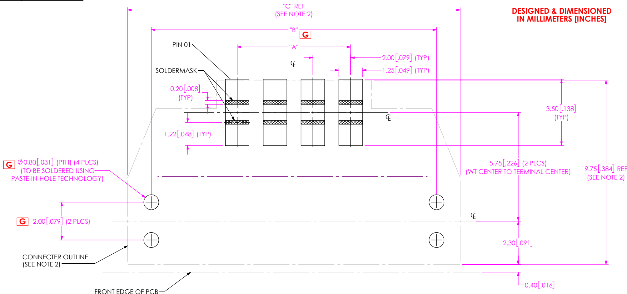
FIG 1 UMPT-04-01-XX-RA-X-WT FOOTPRINT SHOWN
