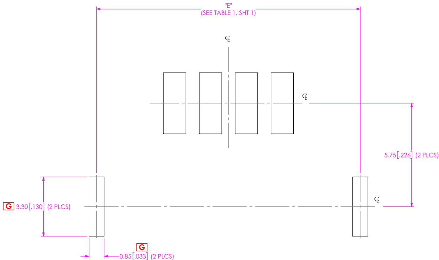
FIG 4 UMPT-04-01-XX-RA-X-WS STENCIL SHOWN (DIFFERENT AS SHOWN, OTHERWISE SAME AS FIG 1 & 3)
