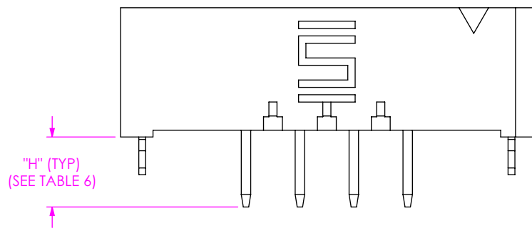
FIG 9 UMPT-04-01.5-XX-V-1-W-XR SHOWN (DIFFERENT AS SHOWN, OTHERWISE SAME AS FIG 2)
