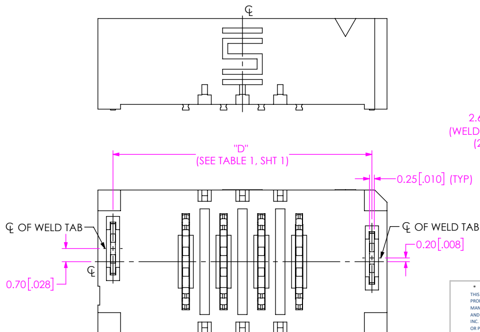
FIG 10 UMPT-04-01.5-XX-V-S-S-XR SHOWN (DIFFERENT AS SHOWN, OTHERWISE SAME AS FIG 2)
