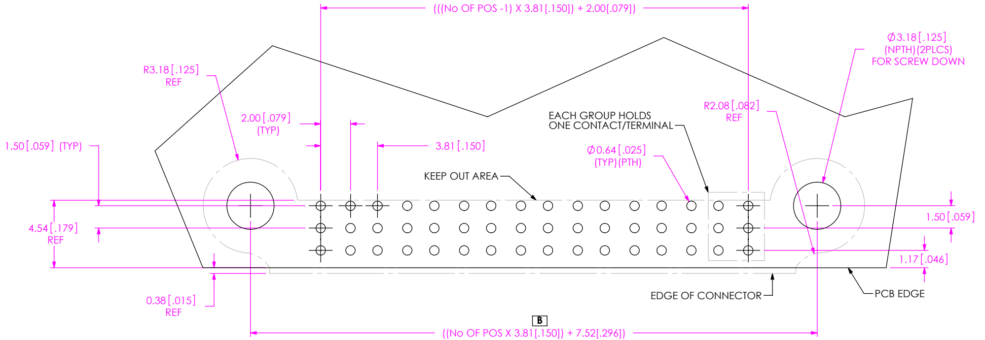
FIG 1 (UPPT-08-01-XX-X-RA-SD-TR SHOWN)
