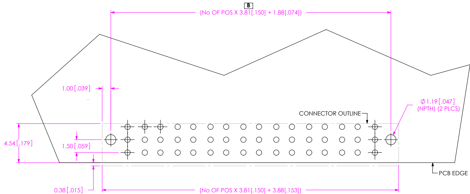
FIG 2 (*UPPT-08-01-XX-X-RA-LC-TR SHOWN)
