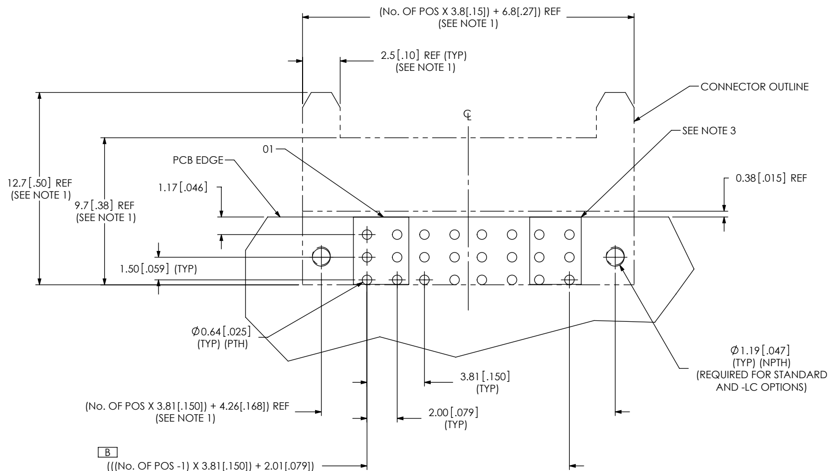
FIG. 1 (UPS-04-XX-X-RA-XX SHOWN)
