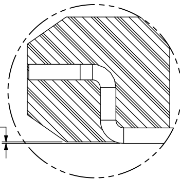
DETAIL 'D' SCALE 20:1
