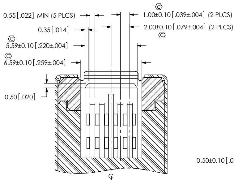
SECTION "B"-"B" SCALE 4:1
