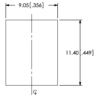
SUGGESTED PANEL CUTOUT DIMENSIONS
