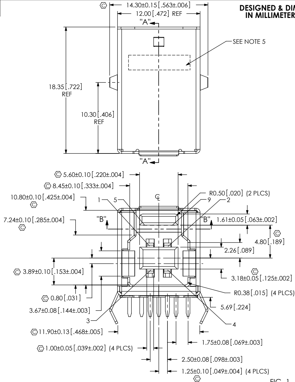
FIG. 1 (USB3-B-S-X-TH SHOWN)
