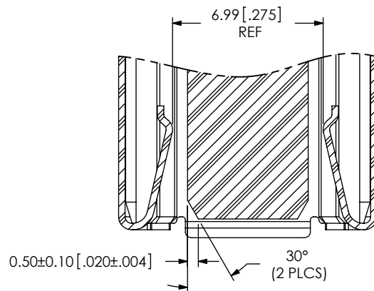
SECTION "C"-"C" SCALE 4:1
