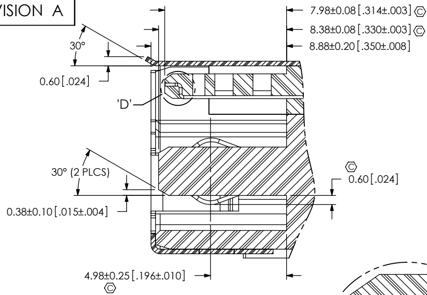
SECTION "A"-"A" SCALE 4:1
