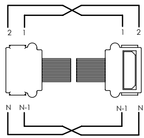
WIRING OPTION 2 POSITION 1 TO POSITION 2
