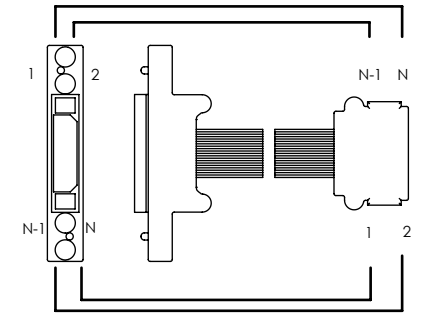
WIRING OPTION 4 POSITION 1 TO POSITION N
