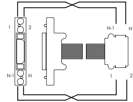
WIRING OPTION 3 POSITION 1 TO POSITIO N-1
