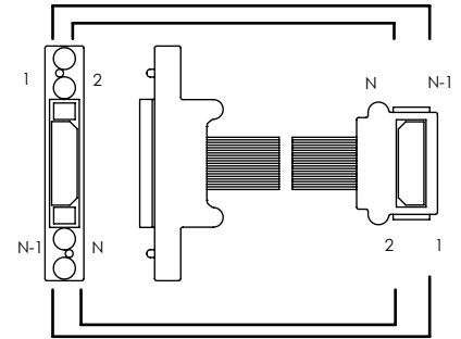
WIRING OPTION 4 POSITION 1 TO POSITION N
