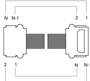
WIRING OPTION 4 POSITION 1 TO POSITION N
