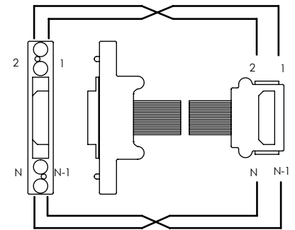
WIRING OPTION 1 POSITION 1 TO POSITION 1
