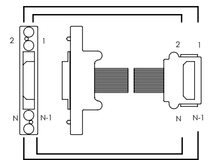
WIRING OPTION 2 POSITION 1 TO POSITION 2
