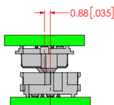
INITIAL Y AXIS LINEAR MISALIGNMENT
