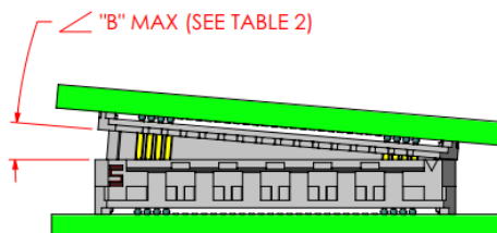
INITIAL Y AXIS ANGULAR MISALIGNMENT
