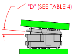
FINAL X AXIS ANGULAR MISALIGNMENT
