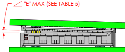
FINAL Y AXIS ANGULAR MISALIGNMENT
