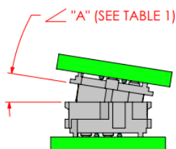
INITIAL X AXIS ANGULAR MISALIGNMENT
