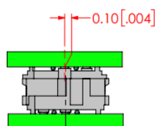
FINAL Y AXIS LINEAR MISALIGNMENT
