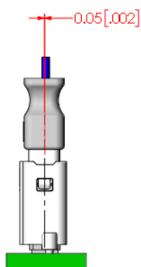
FINAL Y AXIS LINEAR MISALIGNMENT
