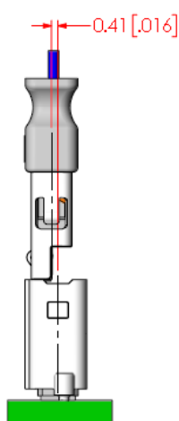
INITIAL Y AXIS LINEAR MISALIGNMENT
