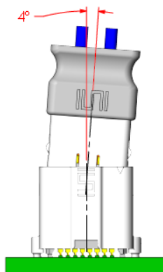
INITIAL Y AXIS ANGULAR MISALIGNMENT
