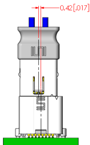
INITIAL X AXIS LINEAR MISALIGNMENT
