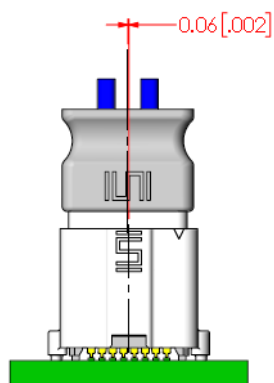
FINAL X AXIS LINEAR MISALIGNMENT
