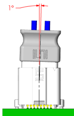
FINAL Y AXIS ANGULAR MISALIGNMENT
