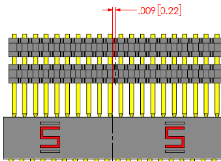
INITIAL X AXIS LINEAR MISALIGNMENT
