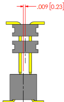
INITIAL Y AXIS LINEAR MISALIGNMENT
