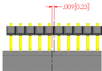
INITIAL X AXIS LINEAR MISALIGNMENT
