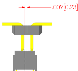
INITIAL Y AXIS LINEAR MISALIGNMENT
