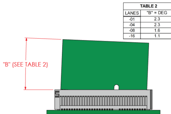
FINAL Y AXIS ANGULAR MISALIGNMENT
