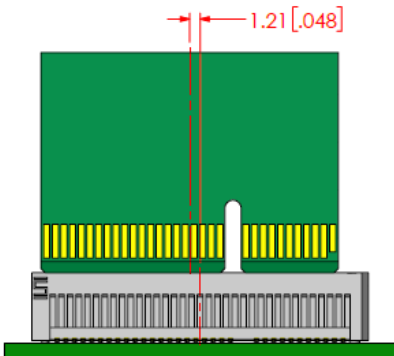
INITIAL X AXIS LINEAR MISALIGNMENT
