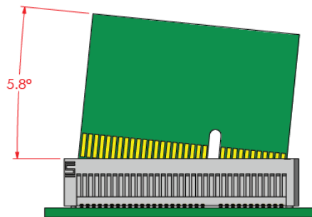
INITIAL Y AXIS ANGULAR MISALIGNMENT
