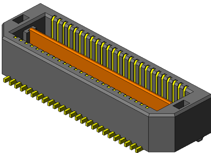
QTS Series – Terminal, Vertical Orientation
