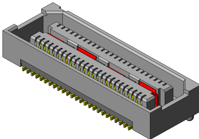
QTS Series – Terminal, Vertical Orientation
