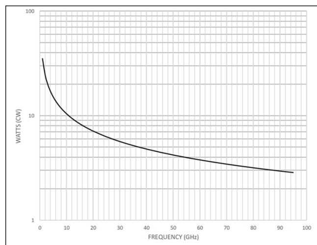
TYPICAL POWER HANDLING @ T=25°C 2
