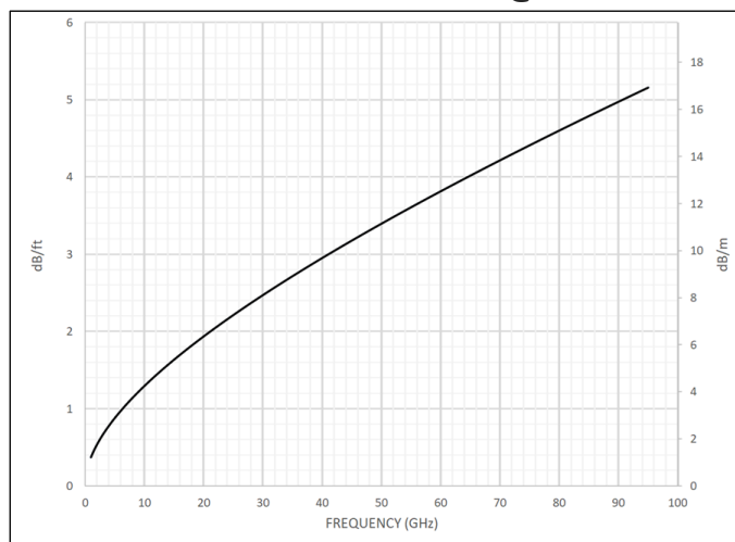
MAXIMUM INSERTION LOSS @ T=25°C 1
