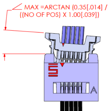
INITIAL Y AXIS ANGULAR MISALIGNMENT
