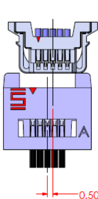
INITIAL X AXIS LINEAR MISALIGNMENT
