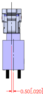
INITIAL Y AXIS LINEAR MISALIGNMENT
