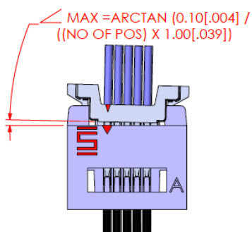
FINAL Y AXIS ANGULAR MISALIGNMENT
