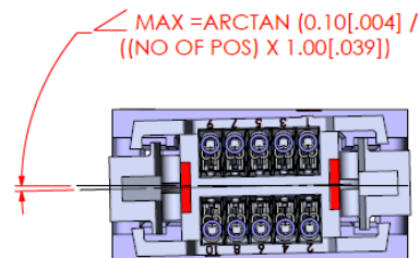
FINAL Z AXIS ANGULAR MISALIGNMENT
