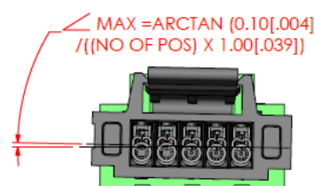
FINAL Z AXIS ANGULAR MISALIGNMENT
