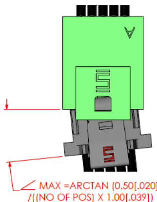
INITIAL Y AXIS ANGULAR MISALIGNMENT
