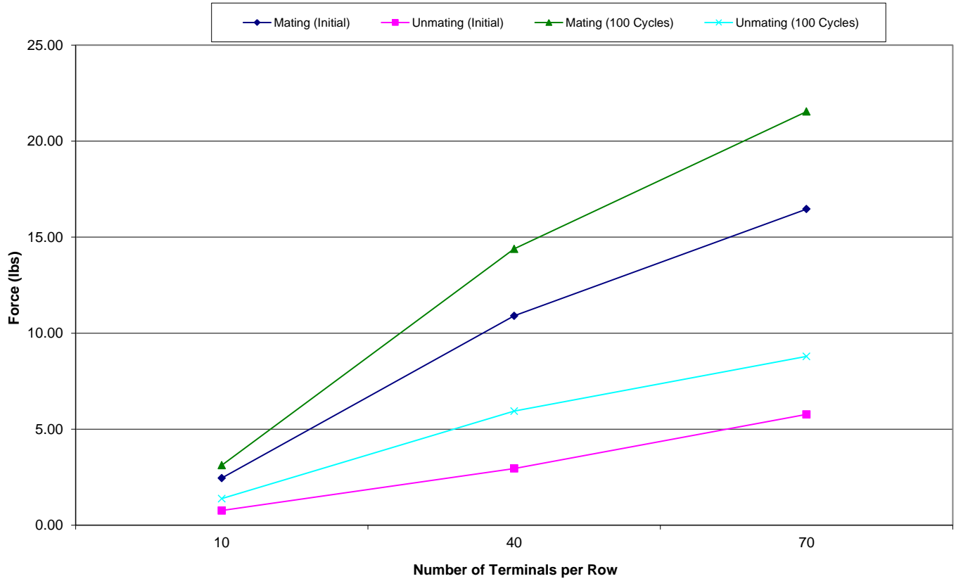
Mating/Unmating Data for 10, 40 and 70 Position HSEC1/CARD
