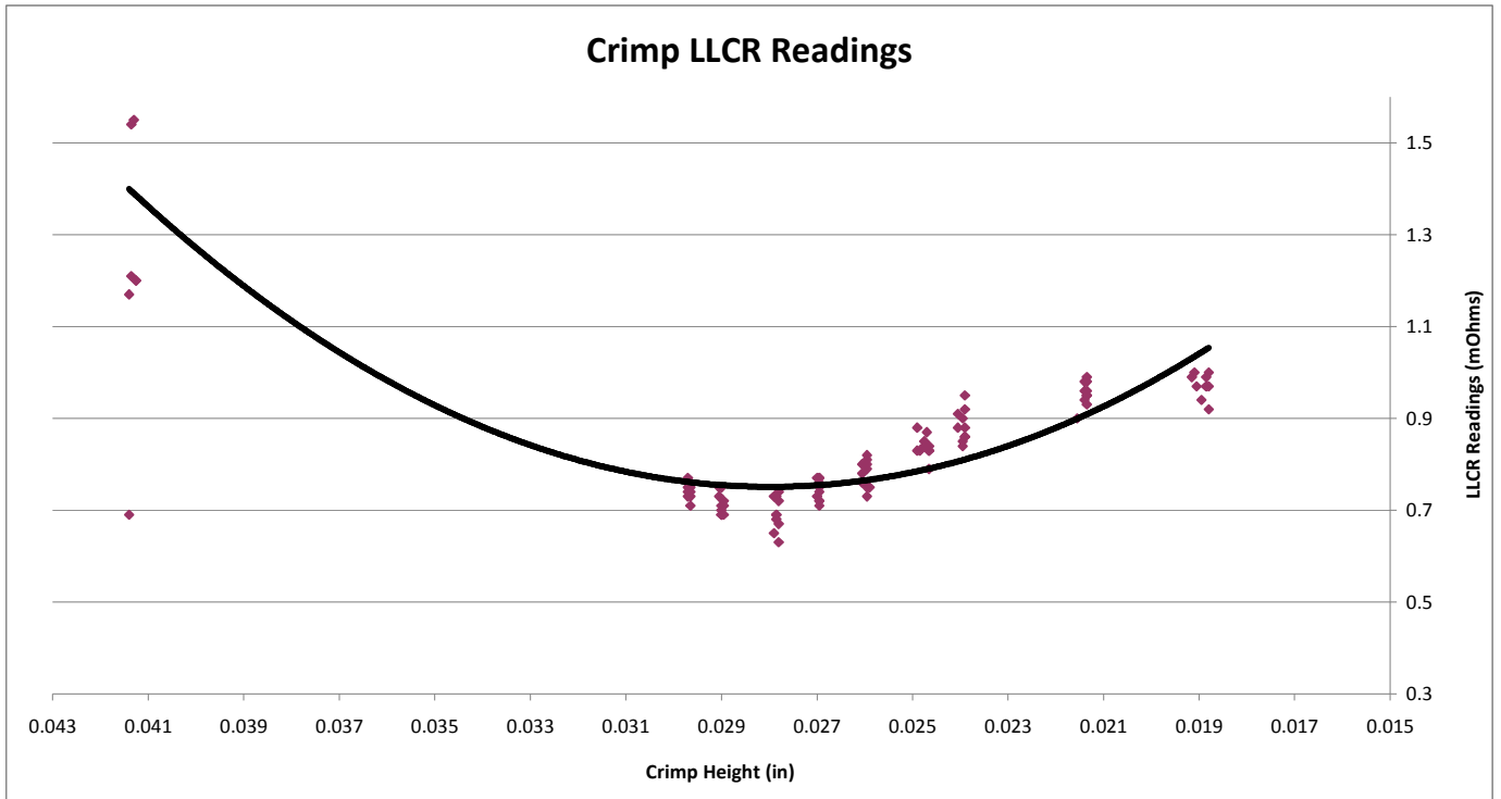
Pull Force Readings
